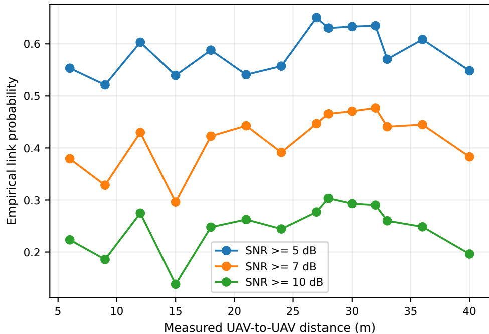
60 GHz A2A beam-scan viability
