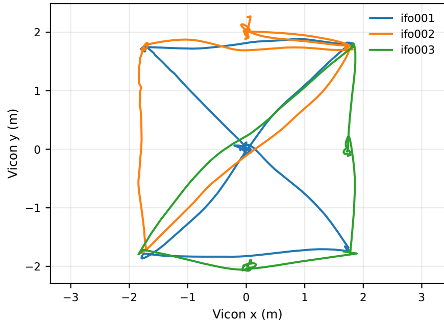
Measured three-UAV motion
