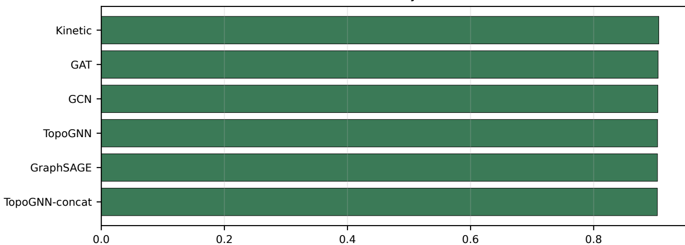
Reachability-delivery proxy (%)
