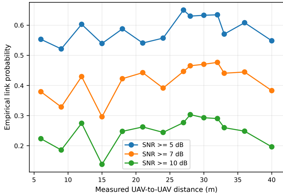
60 GHz A2A beam-scan viability
