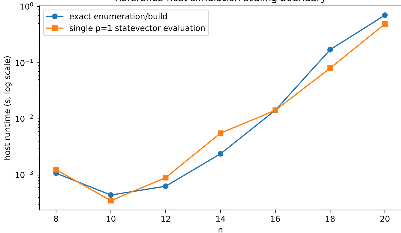
Reference-host simulation scaling boundary
