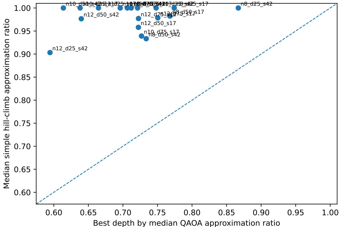
Neutral classical reference on the 18 QAOA instances
