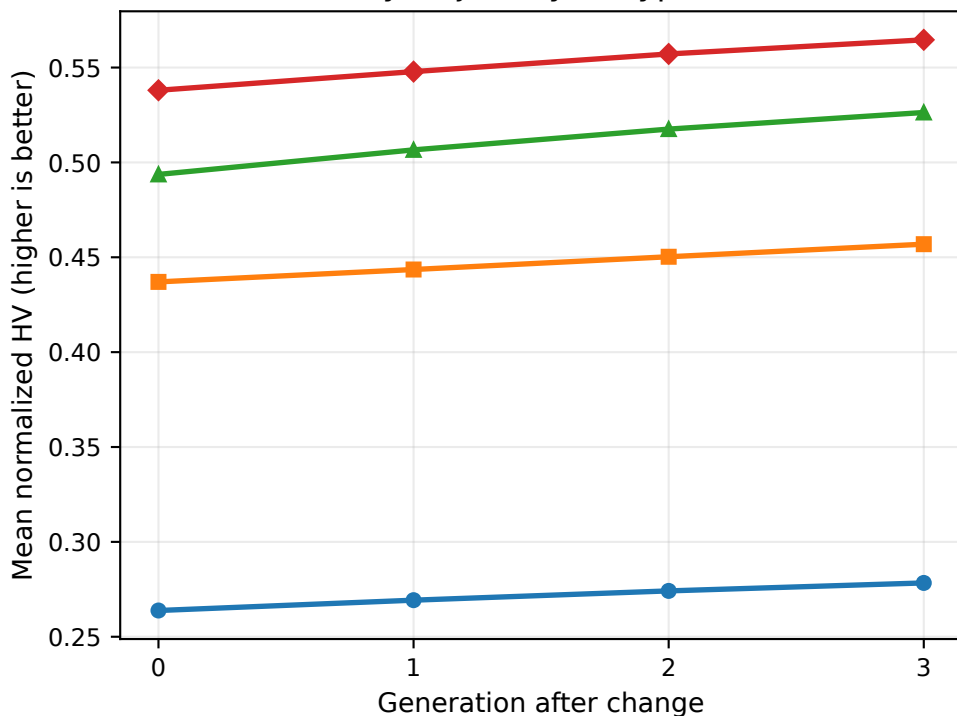
Seven-scenario recovery audit averaged over five common-seed runs and all changed states Recovery trajectory in hypervolume
