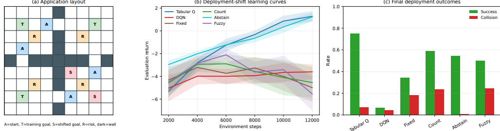
Figure 5: Application-inspired navigation under deployment goal shift. Panel (a) shows the controlled map: starts, recurring training goals, shifted deployment goals, risk cells, and walls. Panels (b) and (c) report learning curves and final deployment outcomes.
