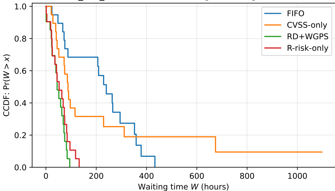
S2_kev_burst: CCDF of waiting time (High bucket)
