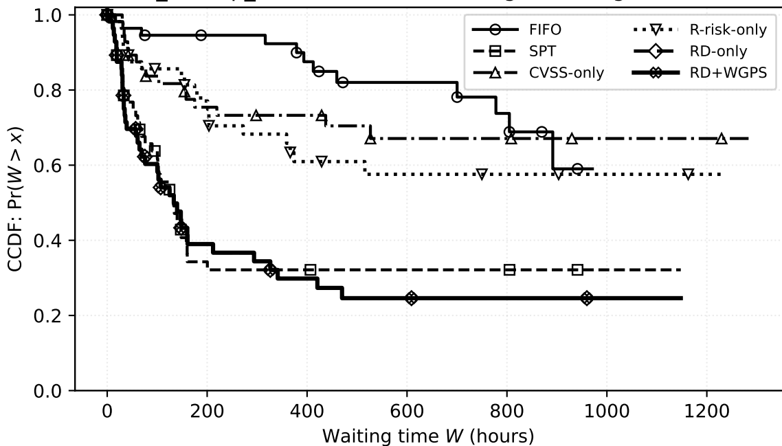
S3_lowcap_hetero: CCDF of waiting time (High bucket)
