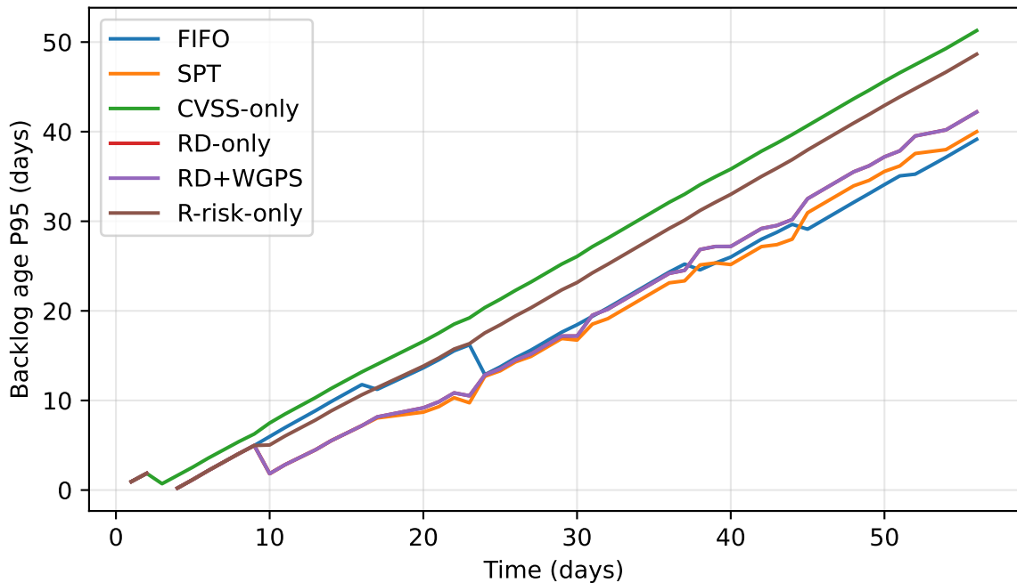
S3: High-bucket backlog age (P95)
