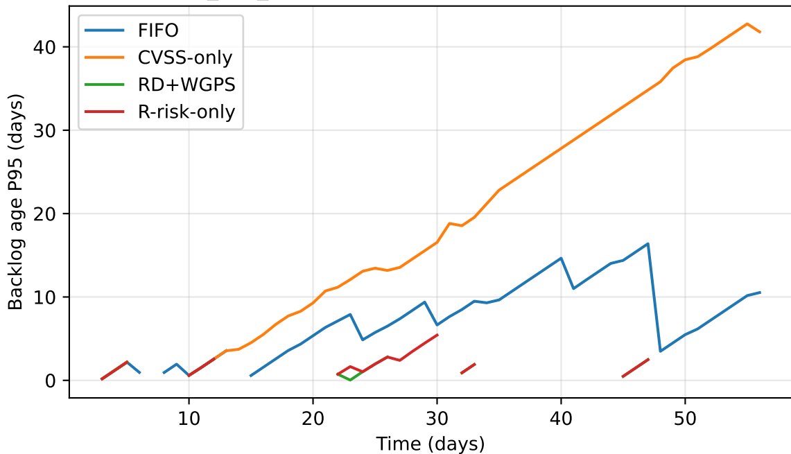
S2_kev_burst: High-bucket backlog age (P95)
