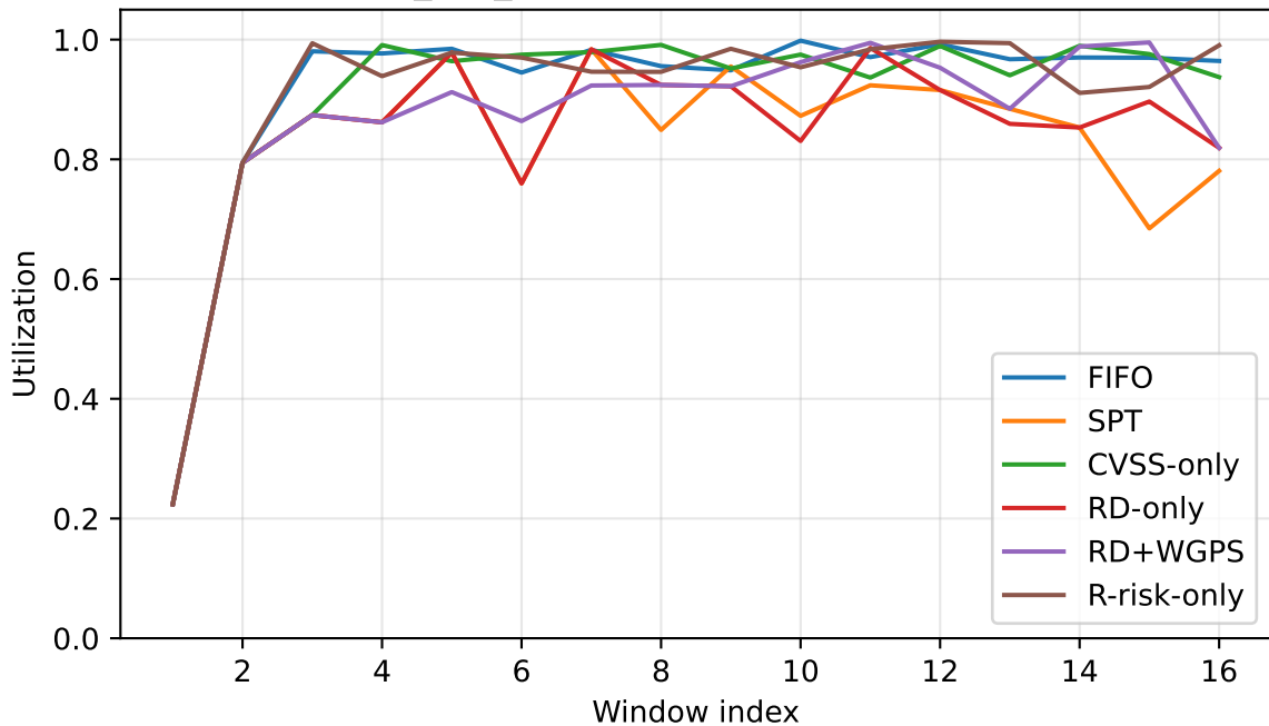
S2_kev_burst: Utilization per window
