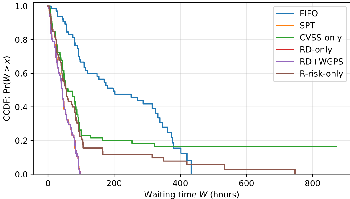
S1: CCDF of waiting time W (High bucket)
