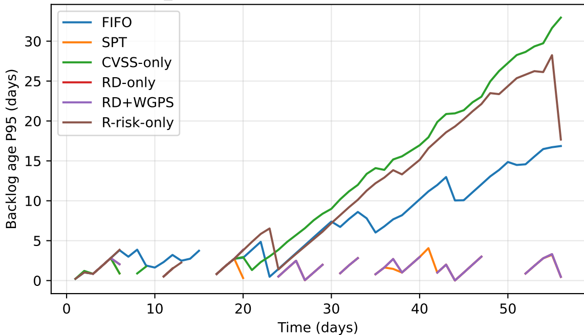
S1_normal: High-bucket backlog age (P95)
