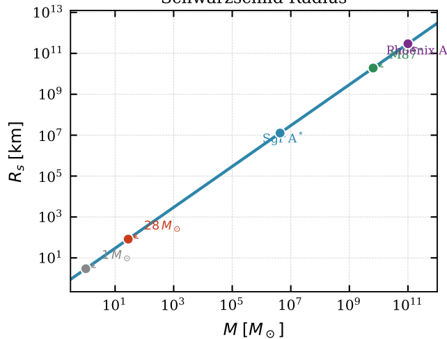
Schwarzschild Radius
