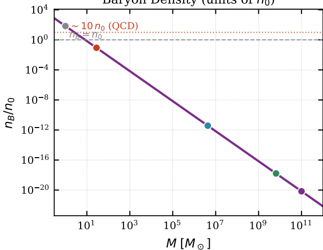
Baryon Density (units of n_0 )
