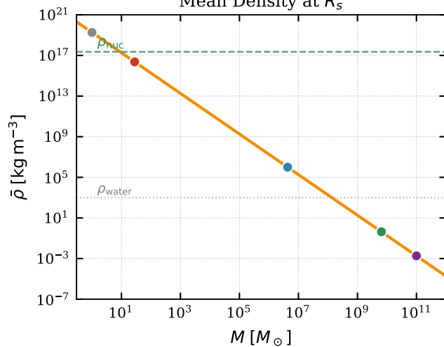
Mean Density at R_s
