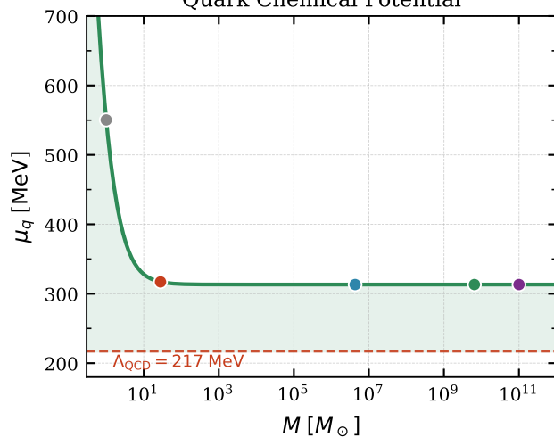
Quark Chemical Potential
