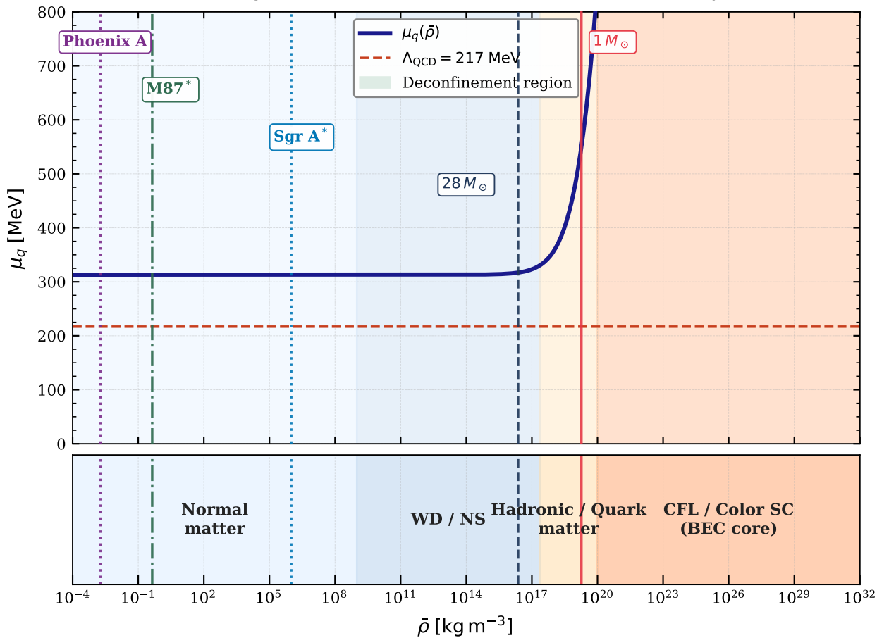
Phase diagram: quark chemical potential vs. mean density at R_5
