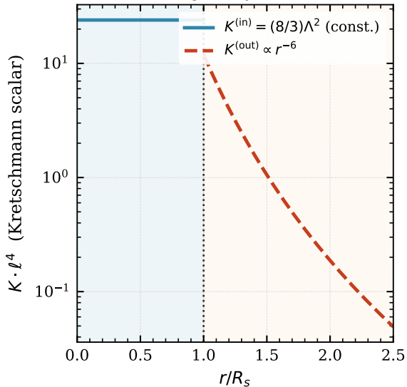
Curvature regularity: K finite at r = 0
