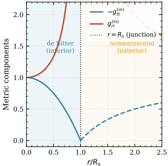
Interior de Sitter + Exterior Schwarzschild
