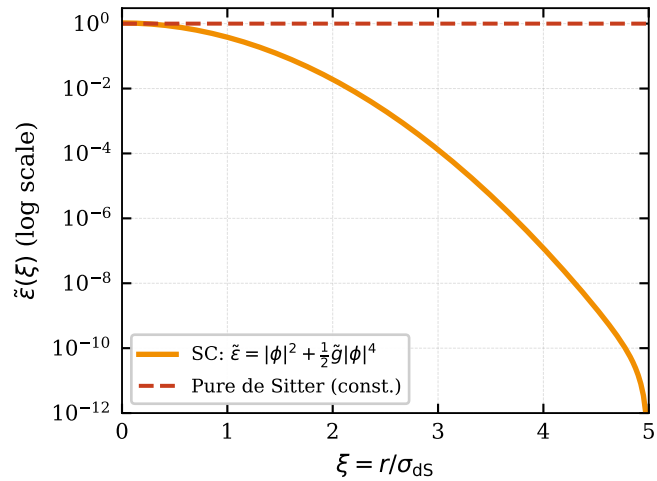
Energy Density: Localized vs. Uniform
