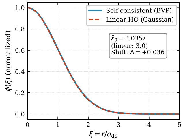
Condensate Profile (Ground State)
