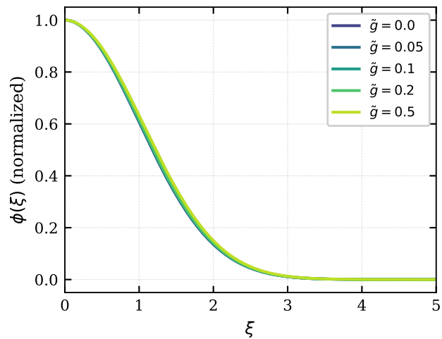
Self-Interaction Effect on Ground State
