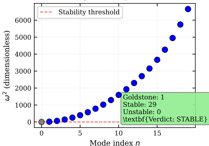
Bogoliubov Spectrum
