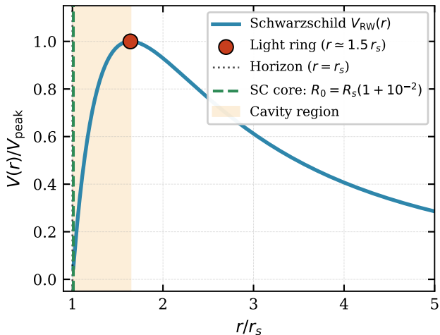
Effective Potential and Cavity
