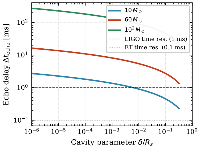
Gravitational Wave Echo Timescale
