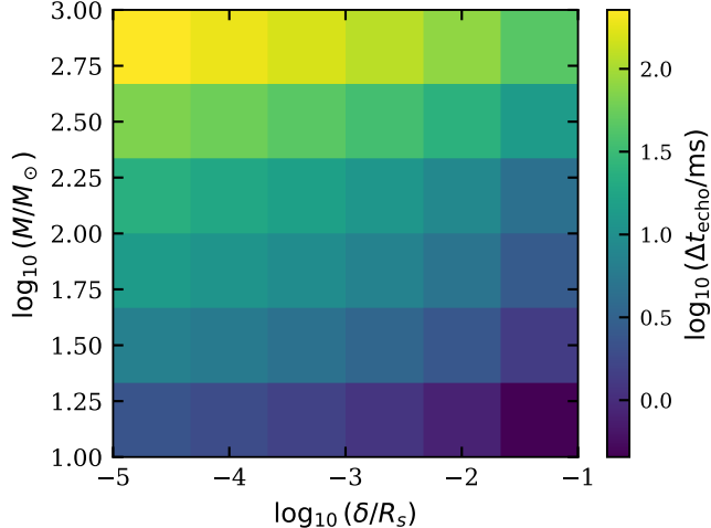
Echo Detectability Map
