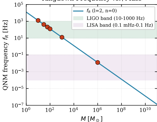
Ringdown Frequency vs. Mass
