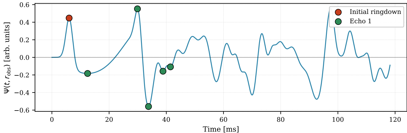
Time-domain gravitational wave echoes from SC cavity Time-Domain Waveform: M = 60 M_{\odot} , \delta/R_s = 10^{-2}
