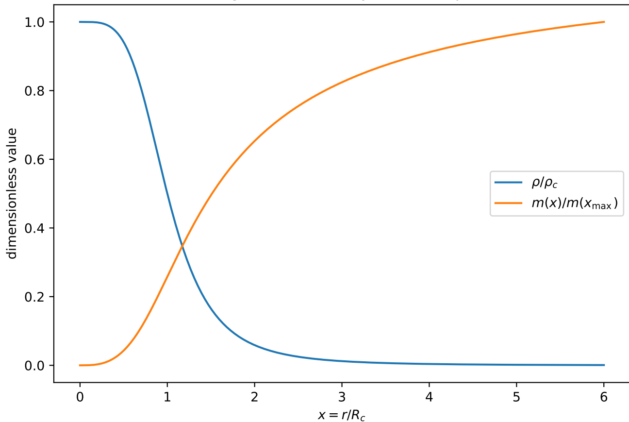
BEY regular-core density and mass profile
