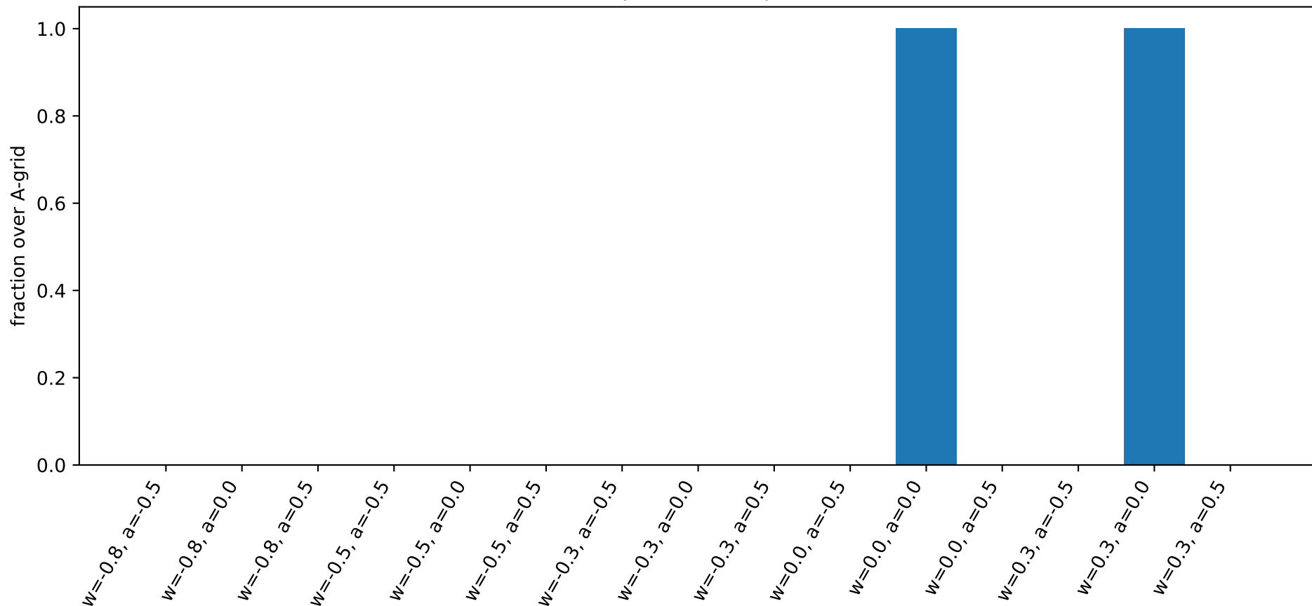
BEY strict acceptance over parameter scan
