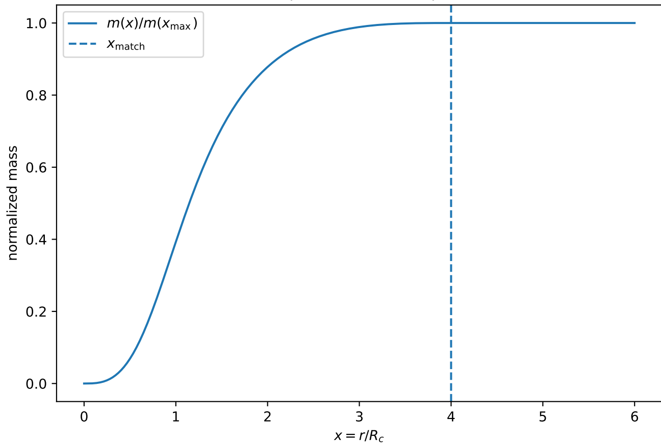
BEY tapered-core mass profile
