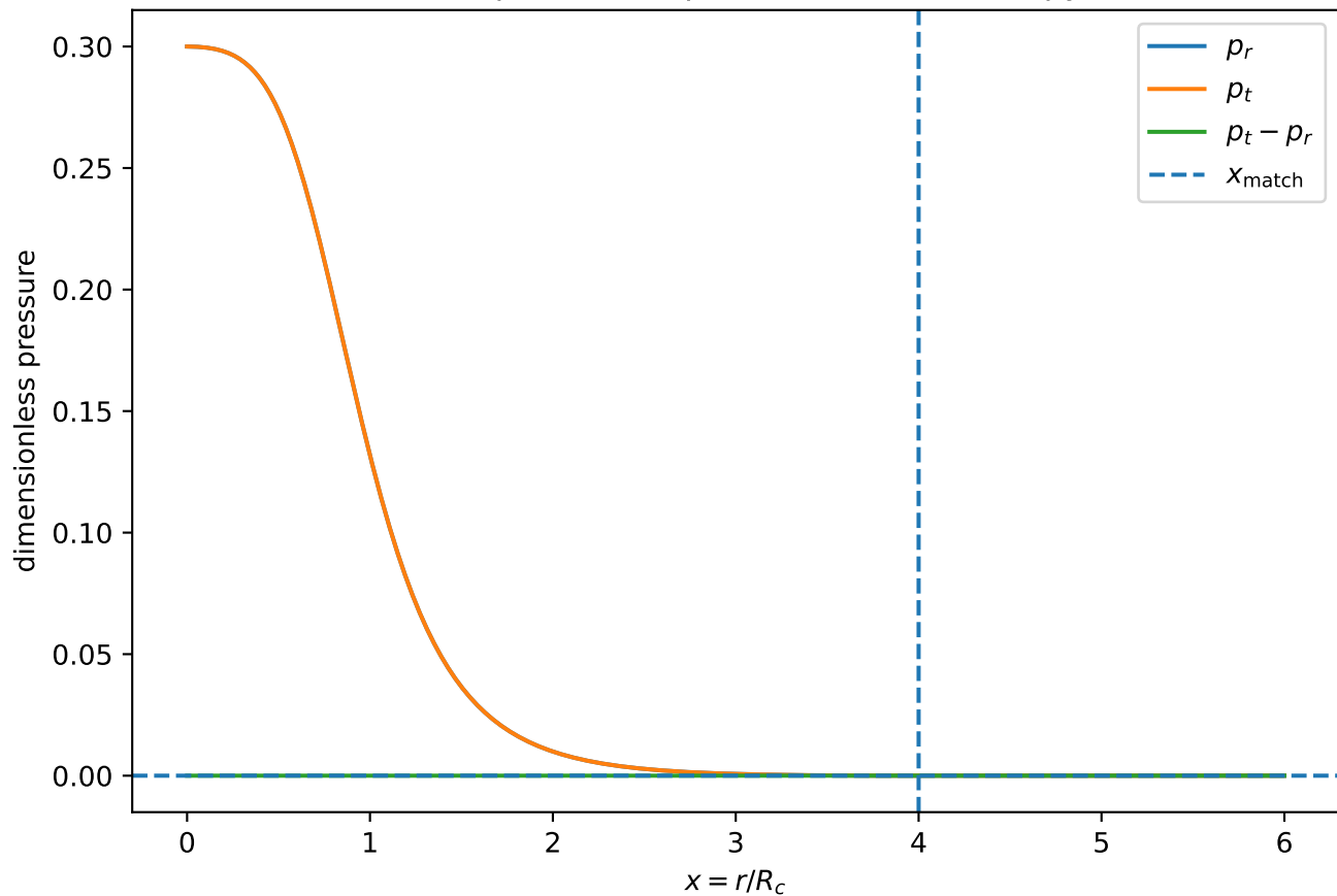
BEY tapered-core pressure and anisotropy
