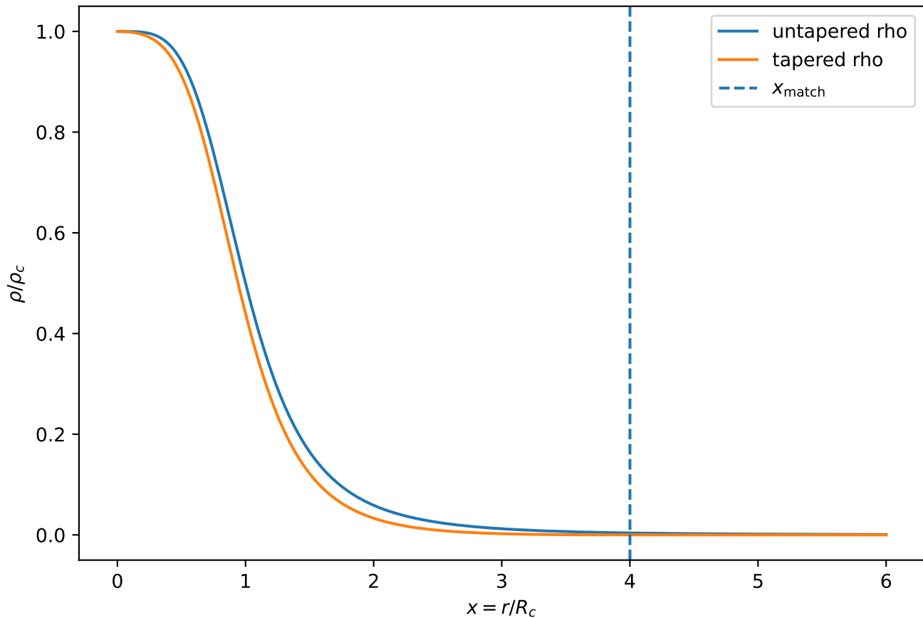
BEY untapered vs tapered boundary density
