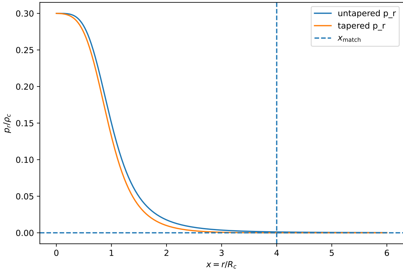
BEY untapered vs tapered boundary pressure
