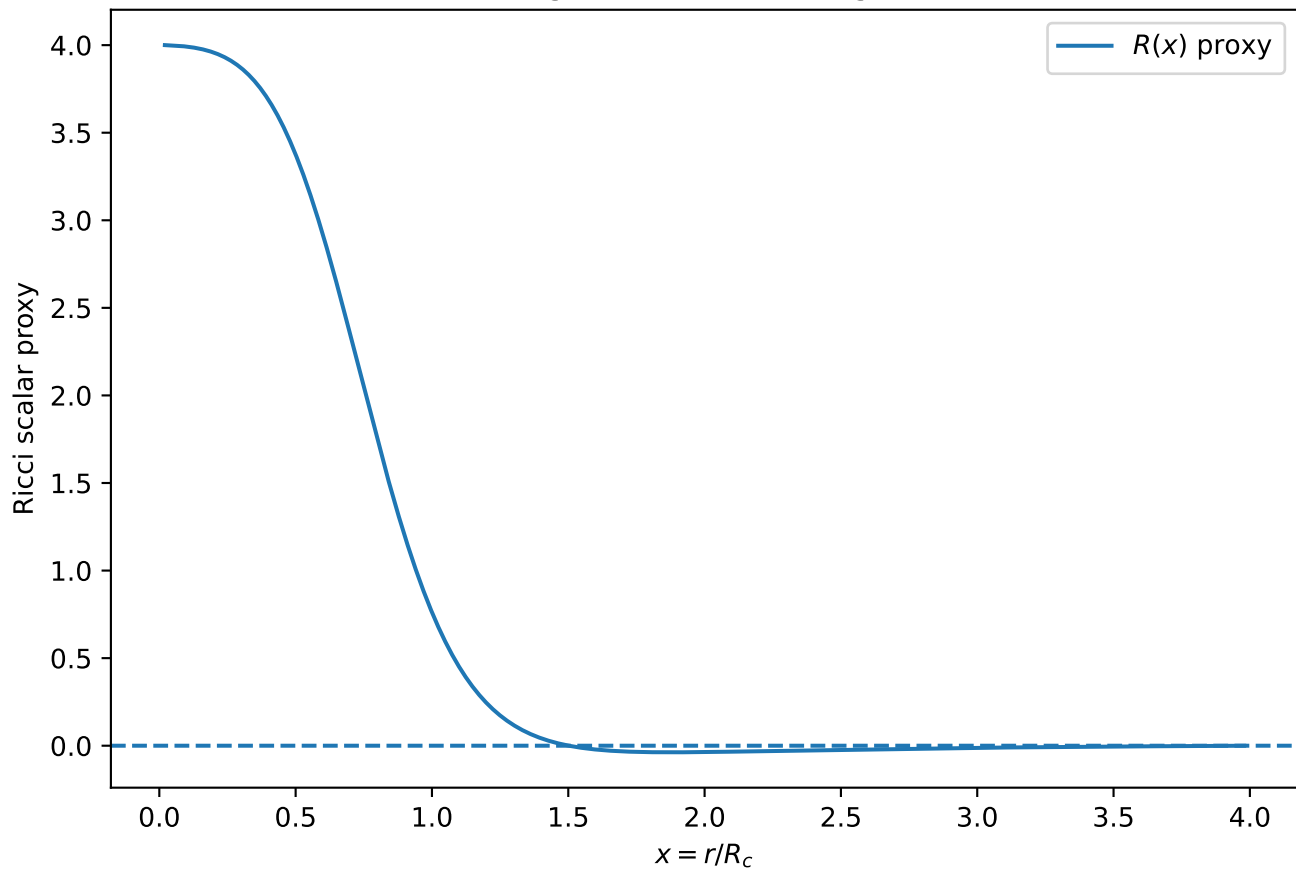
BEY regular-core Ricci diagnostic
