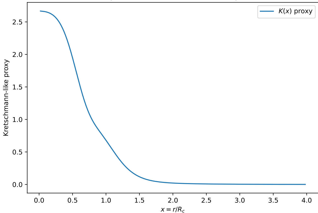
BEY regular-core Kretschmann-like diagnostic
