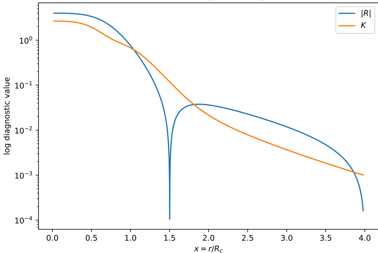
BEY curvature diagnostics, log scale
