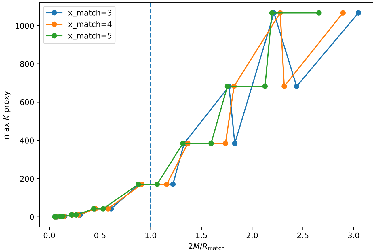
BEY curvature proxy vs compactness
