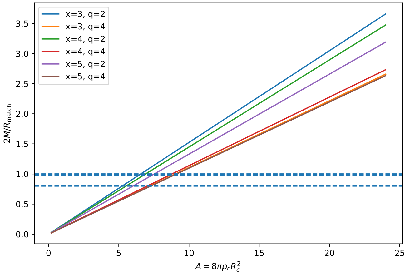
BEY compactness branch map
