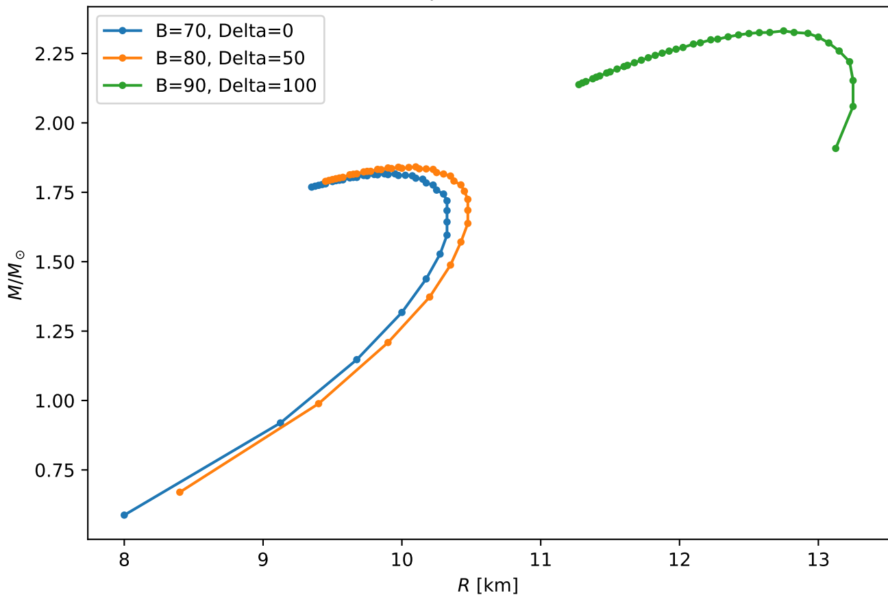
Einstein + QCD-inspired EOS mass-radius curves
