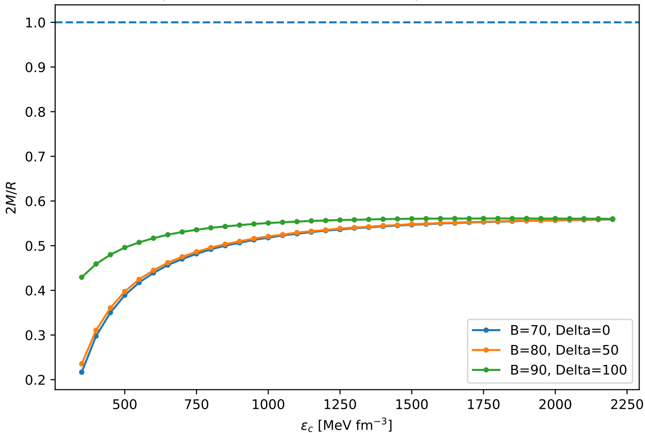
Compactness from Einstein-QCD-inspired TOV solutions
