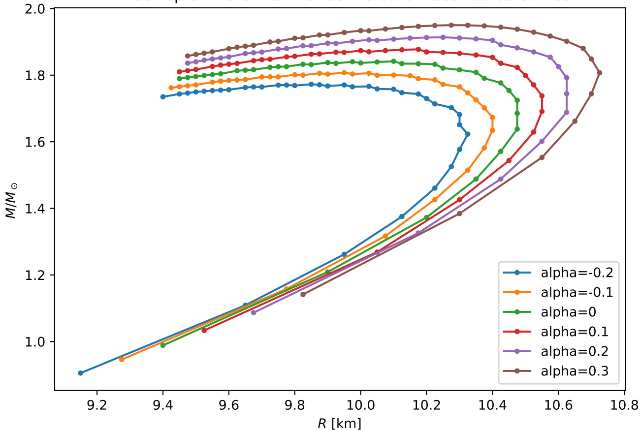
Anisotropic Einstein-CFL effective-core mass-radius curves
