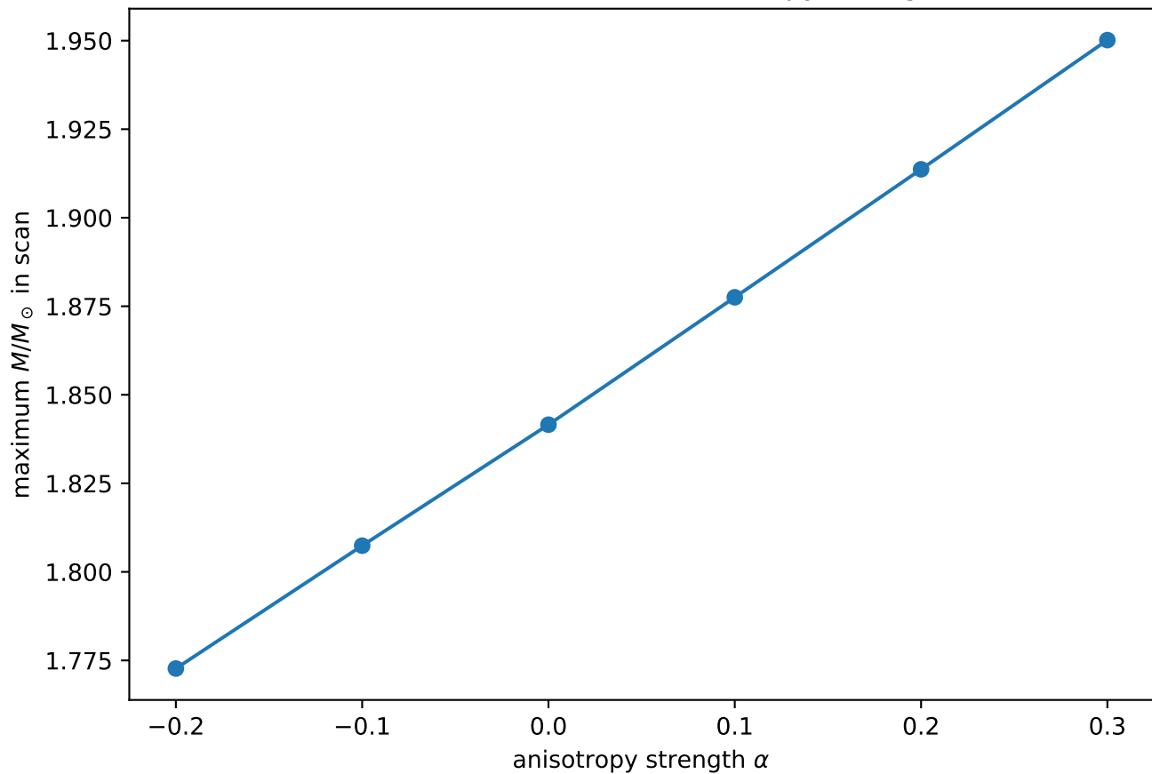
Maximum mass versus anisotropy strength
