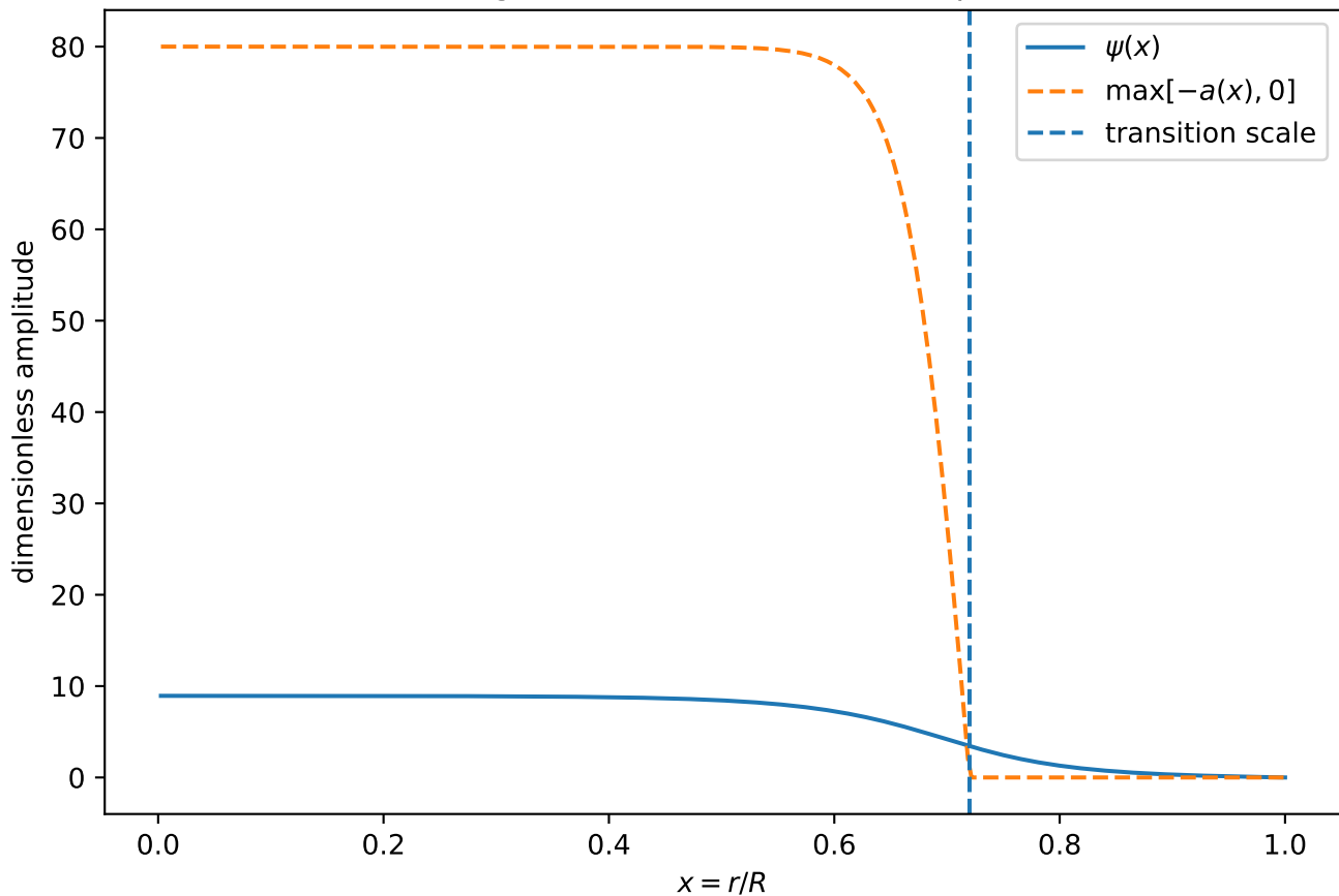
Fixed-background relativistic GL order parameter
