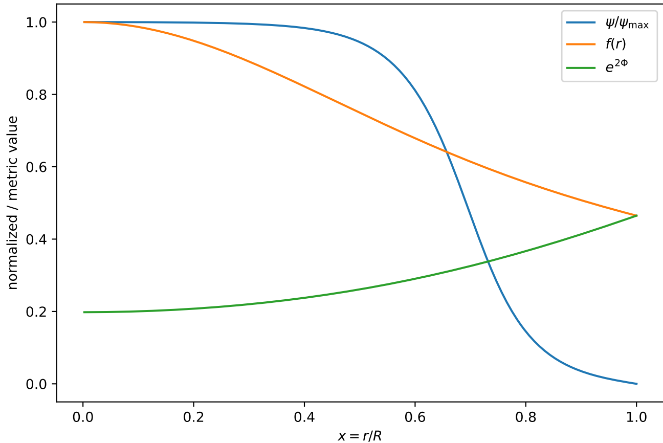
Metric background and GL condensate support
