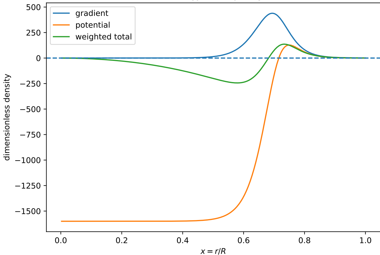
GL free-energy density diagnostics
