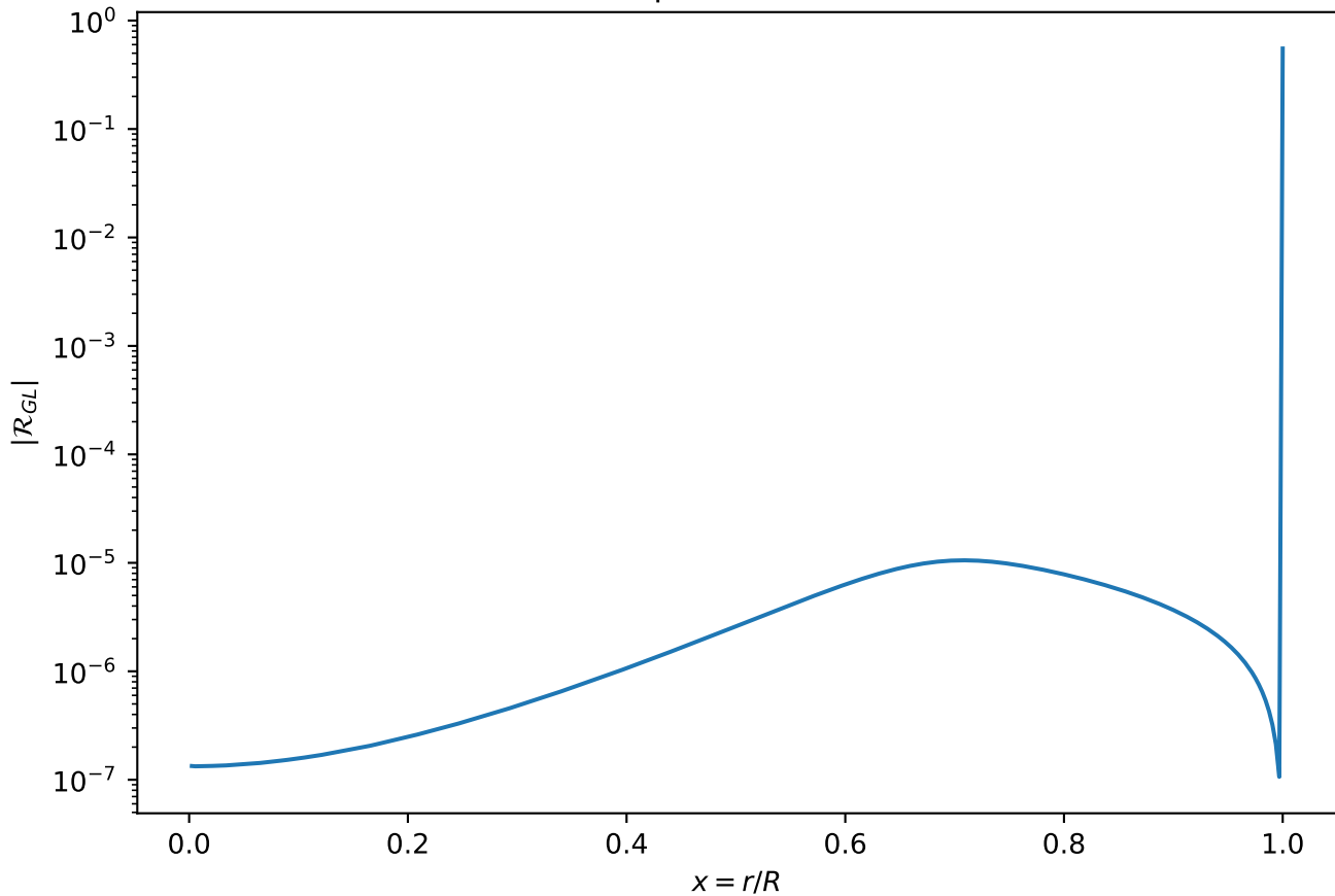
GL equation residual
