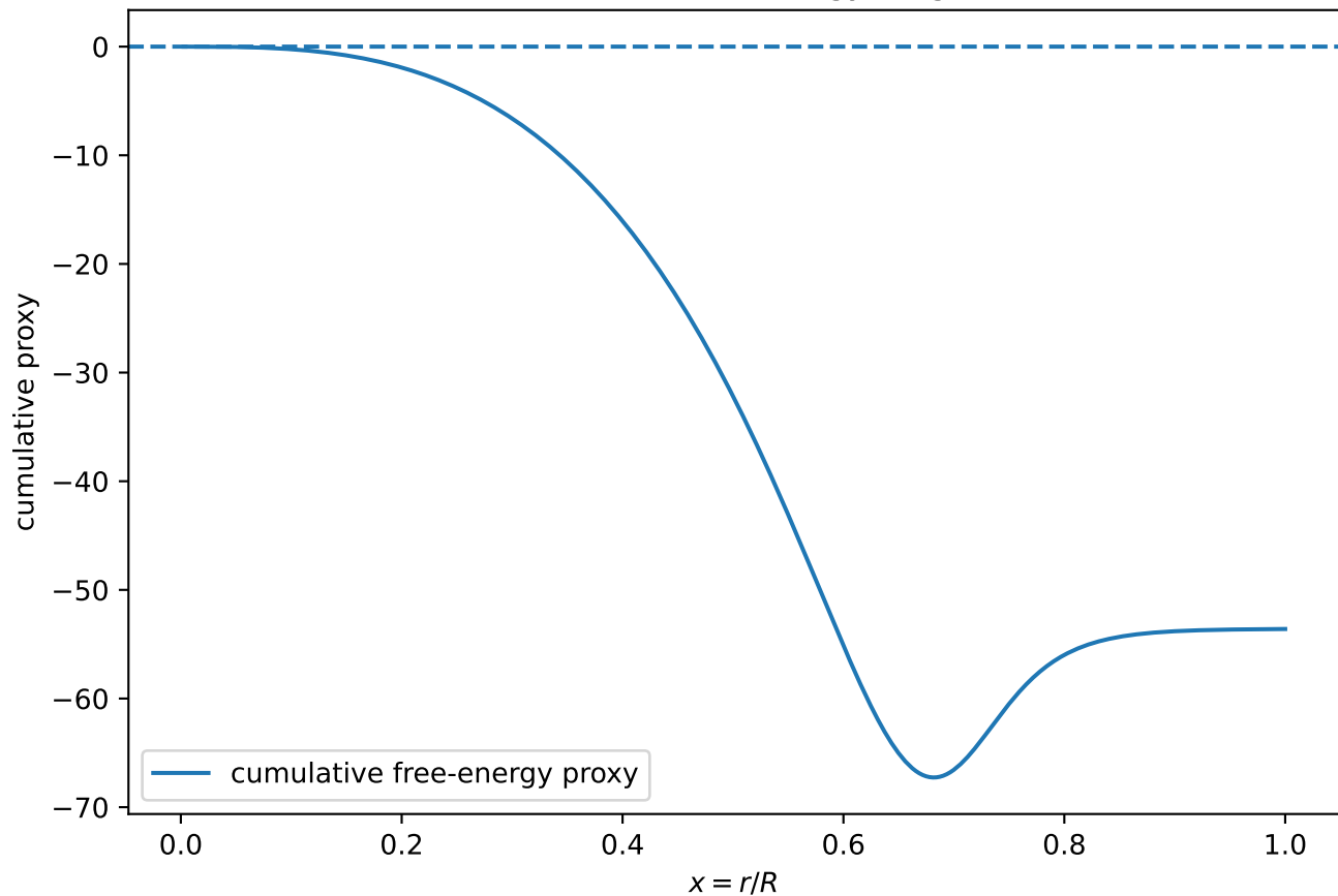
Cumulative GL free-energy diagnostic
