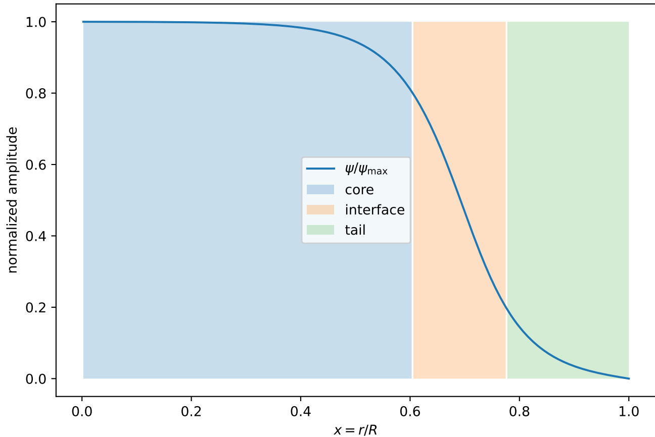
GL condensate core-interface-tail decomposition
