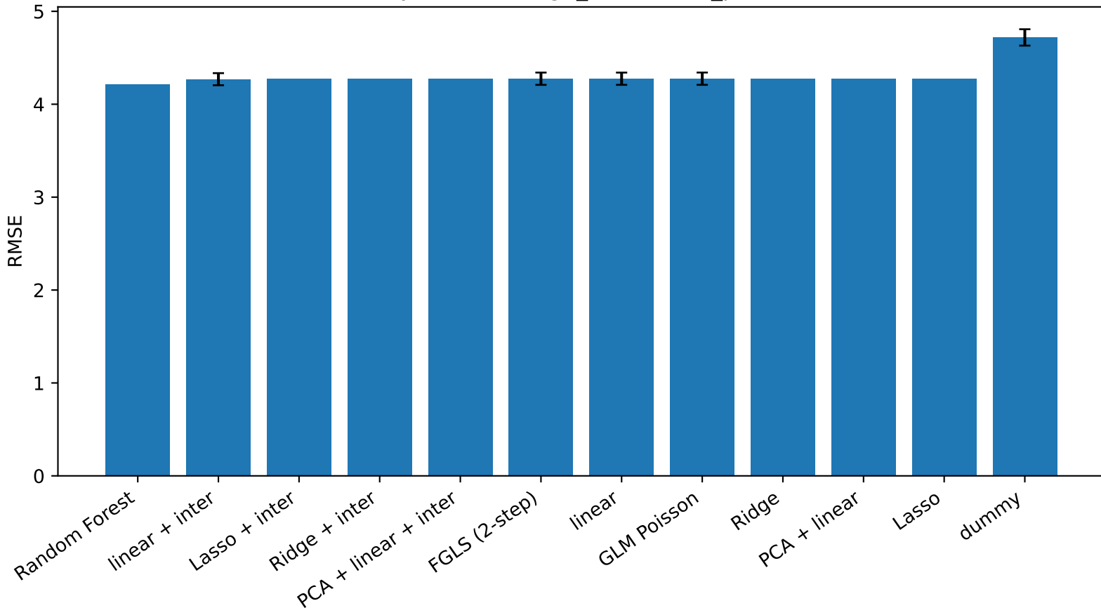
RMSE by model — high_cholesterol_prevalence
