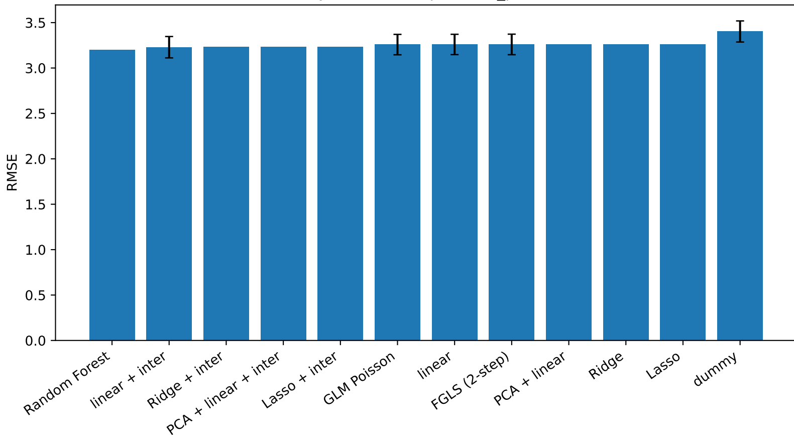
RMSE by model — depression_prevalence
