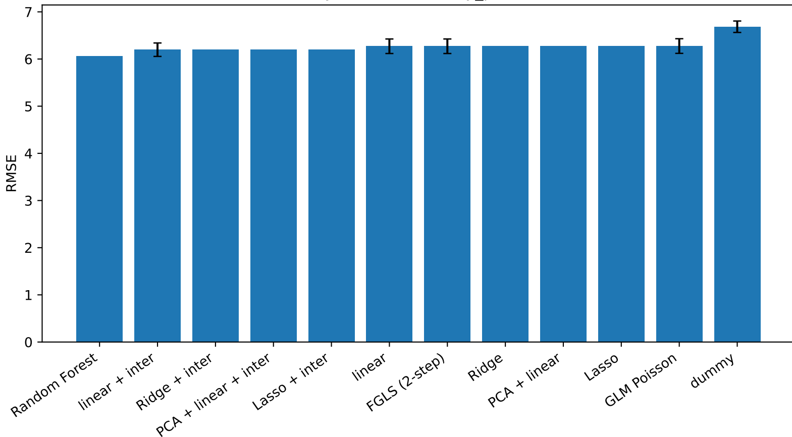
RMSE by model — obesity_prevalence
