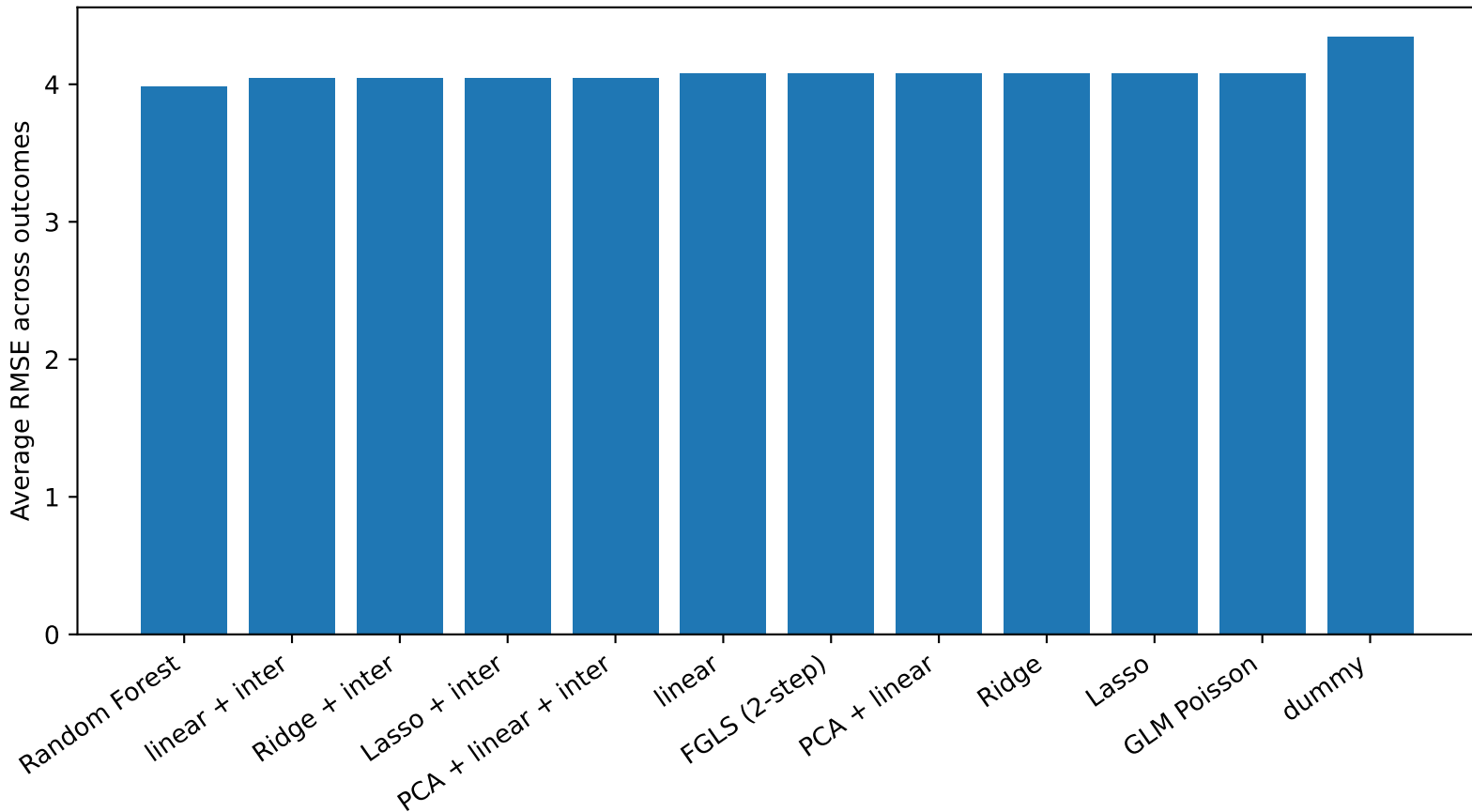
Overall average RMSE by model
