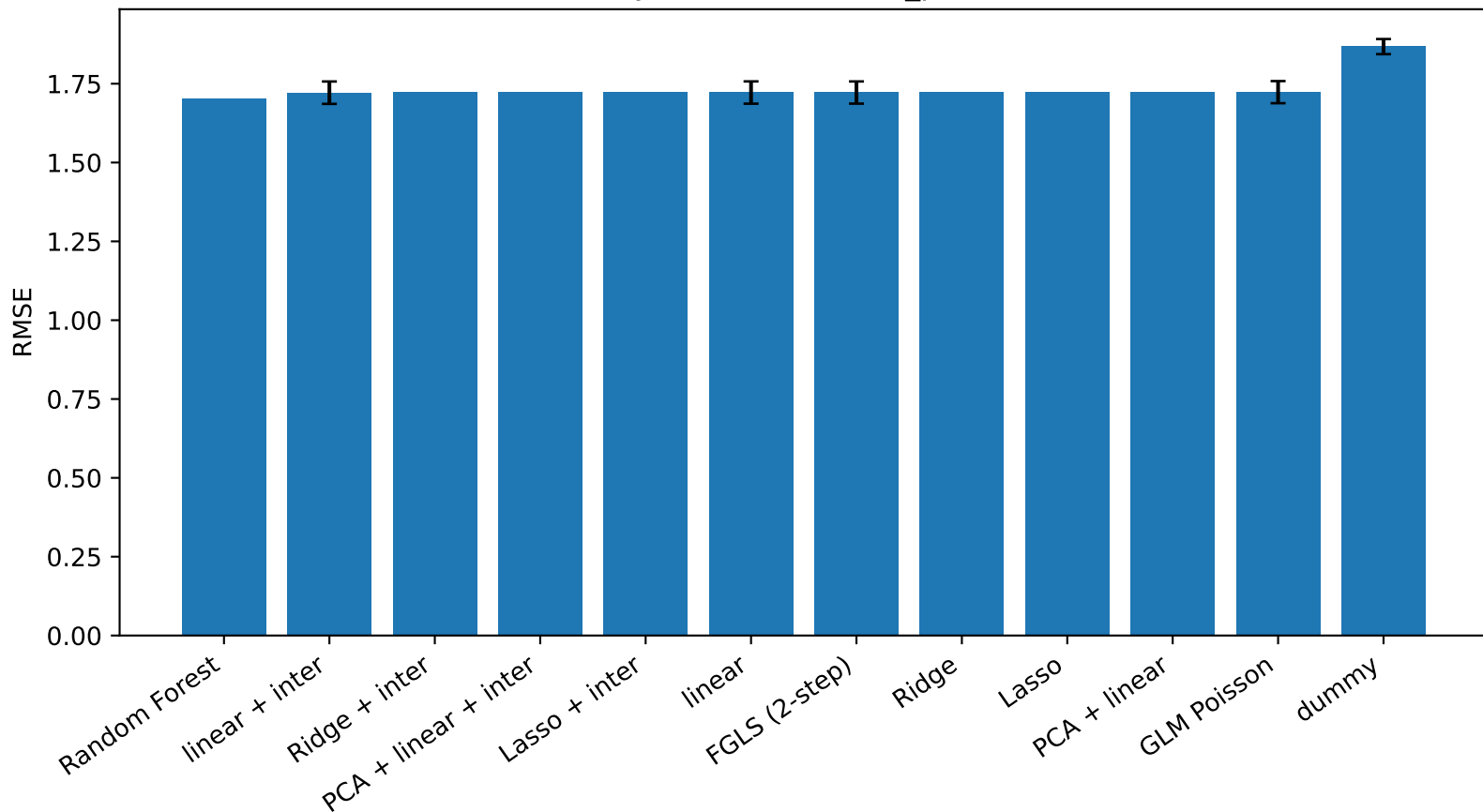
RMSE by model — cancer_prevalence
