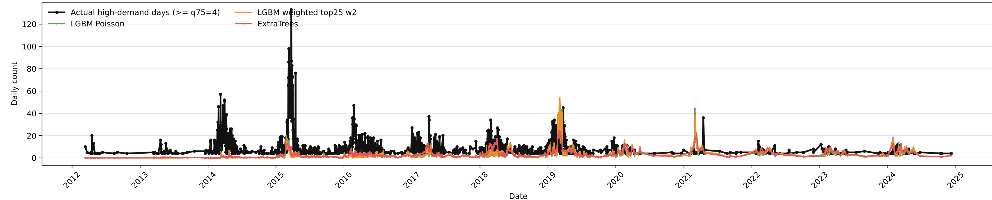
Top-Quartile Actual Demand Days: peak-day predictions remain low
