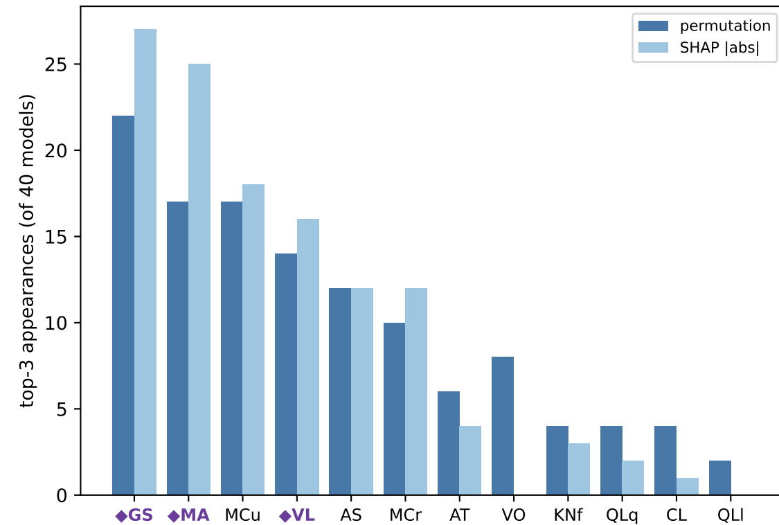
C. How often each dim is top-3, by method (perm-only dims = likely collinearity artifacts)
