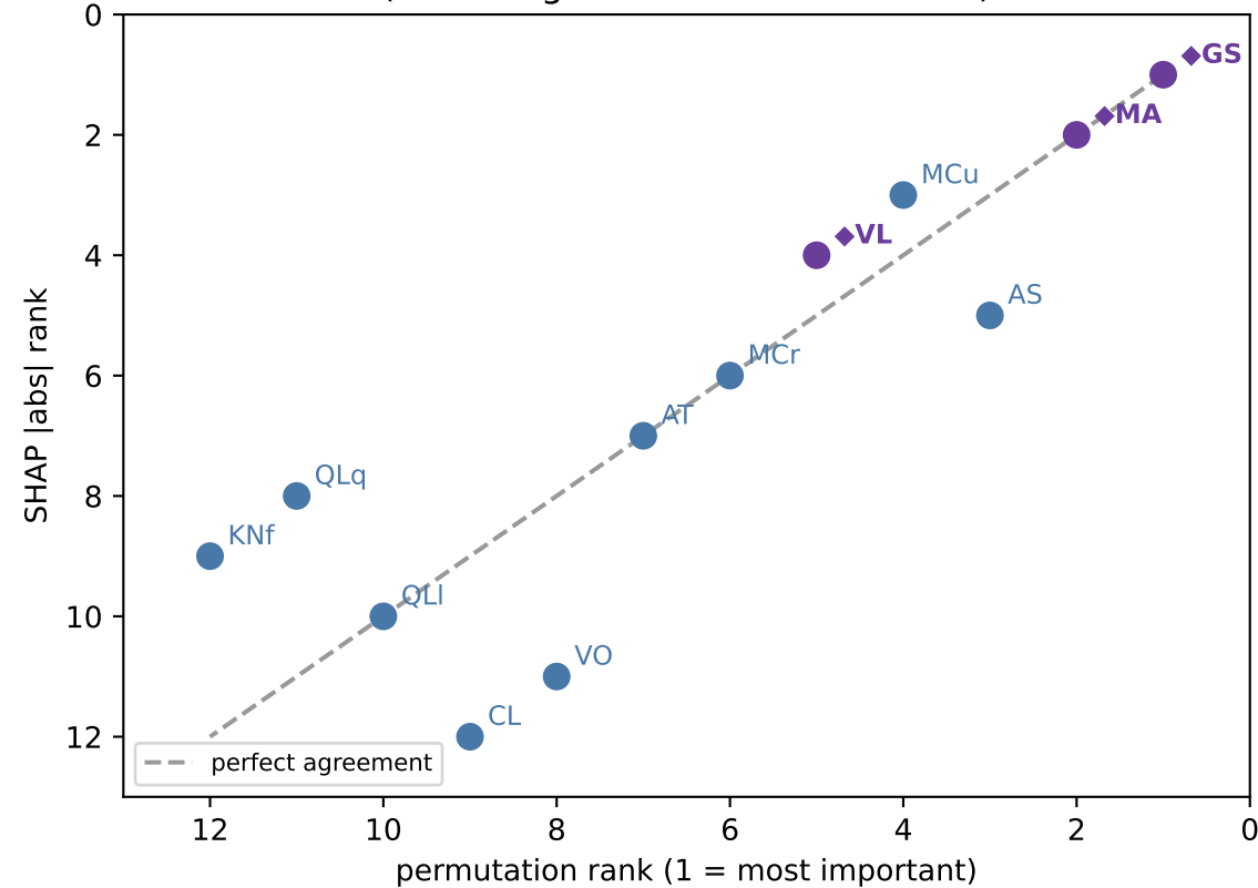
B. COMBINATION_ALL ranking (near diagonal = methods concur)
