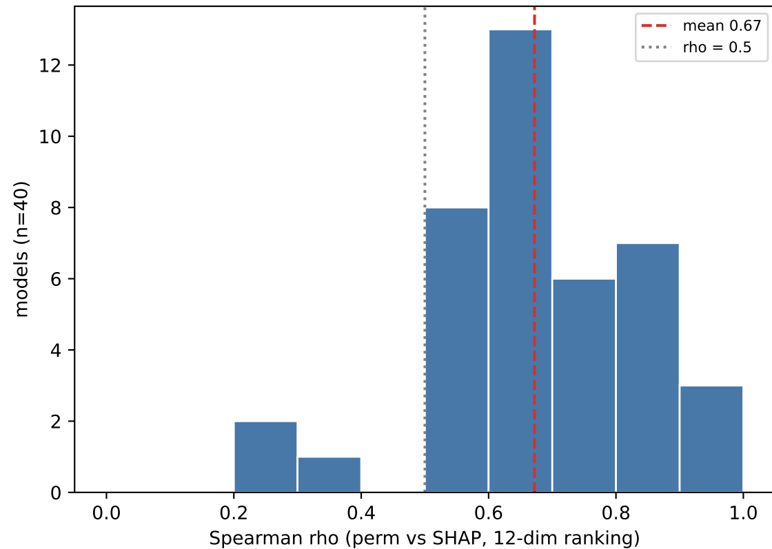
A. Ranking agreement per model 92% of models \rho > 0.5 , top-1 dim matches 68%
