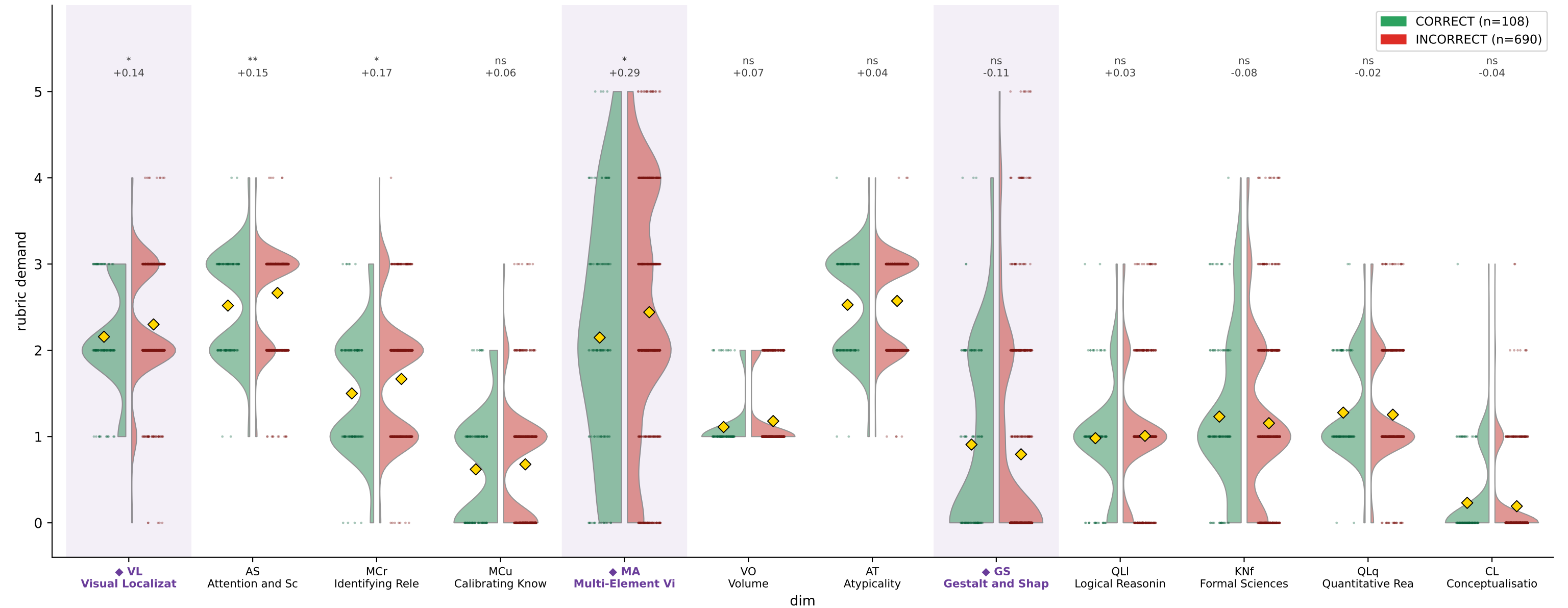
CharXiv DeLeAn demand by reasoning correctness — LLaVA-1-6-Mistral-7B (train)
