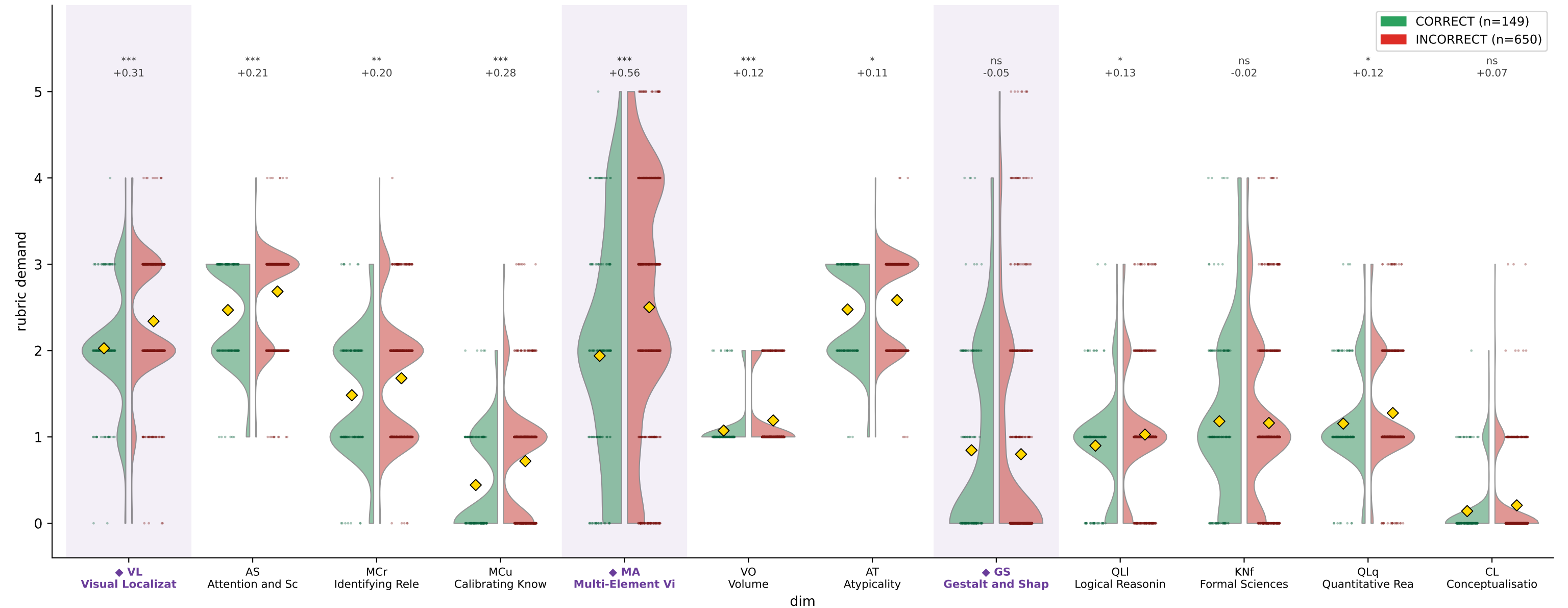
CharXiv DeLeAn demand by reasoning correctness — Mini-Gemini-HD-LLaMA3-8B (train)
