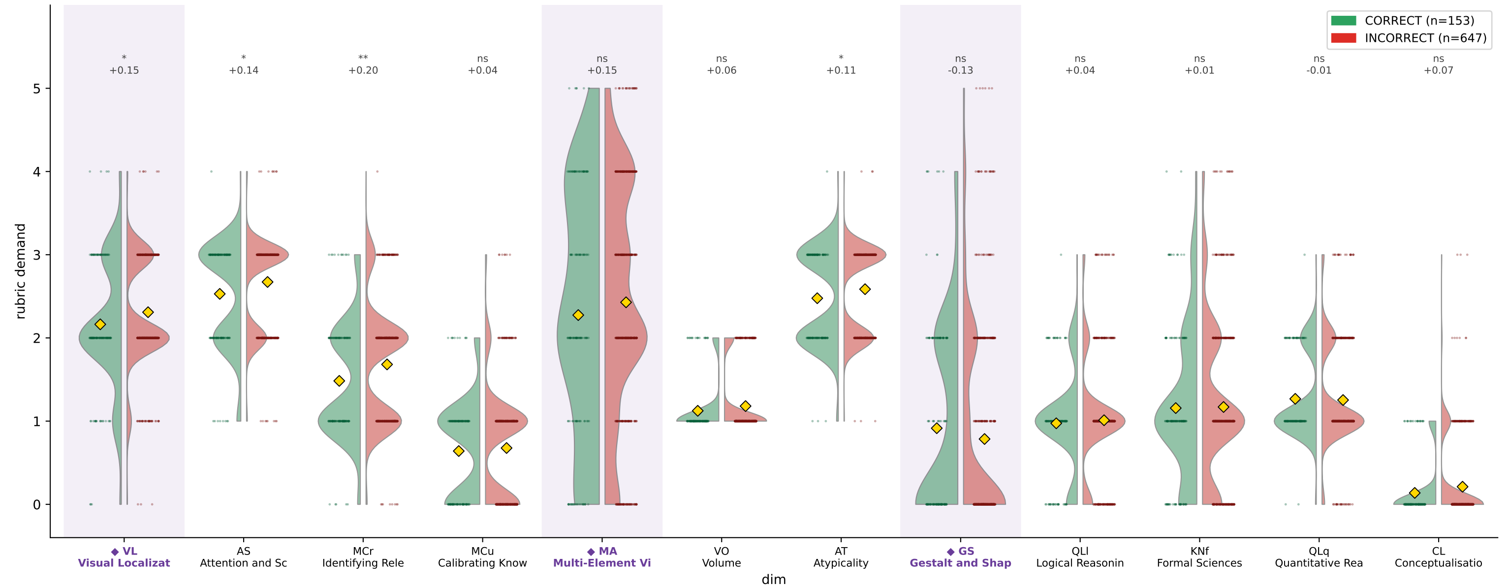
CharXiv DeLeAn demand by reasoning correctness — MoAI (train)
