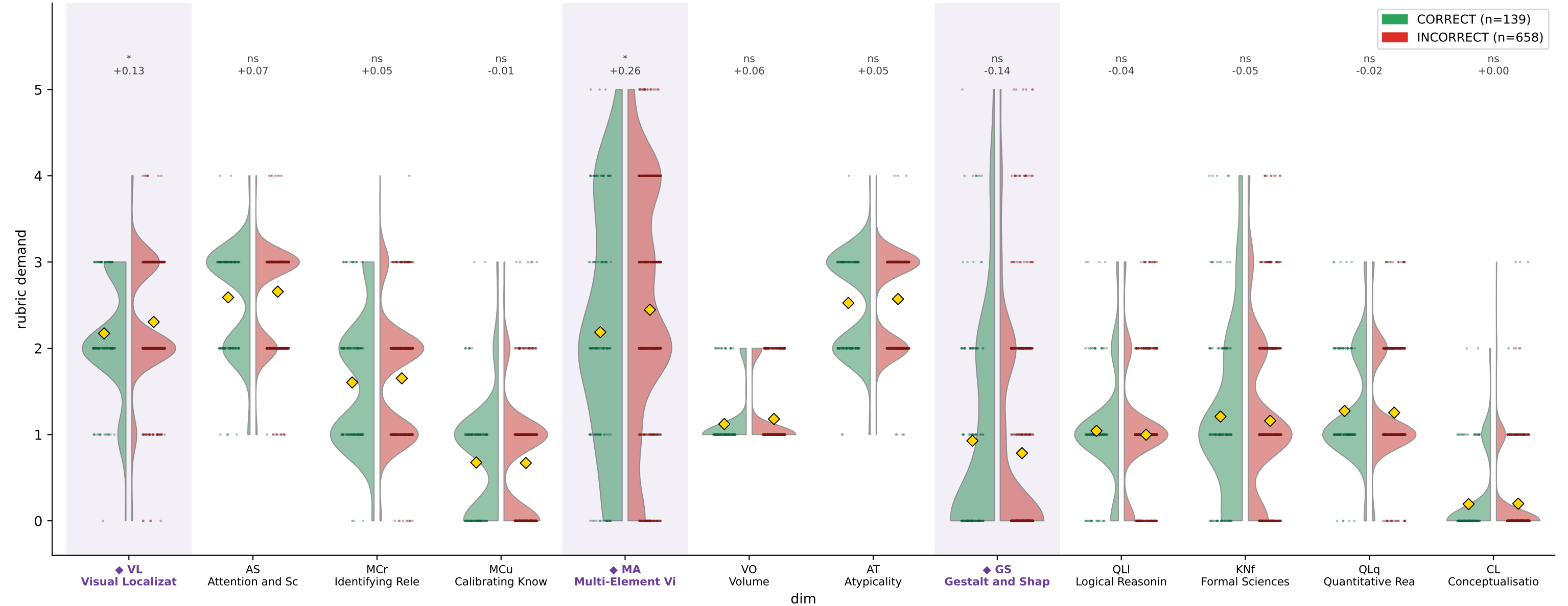
CharXiv DeLeAn demand by reasoning correctness — IDEFICS-2-Chatty (train)
