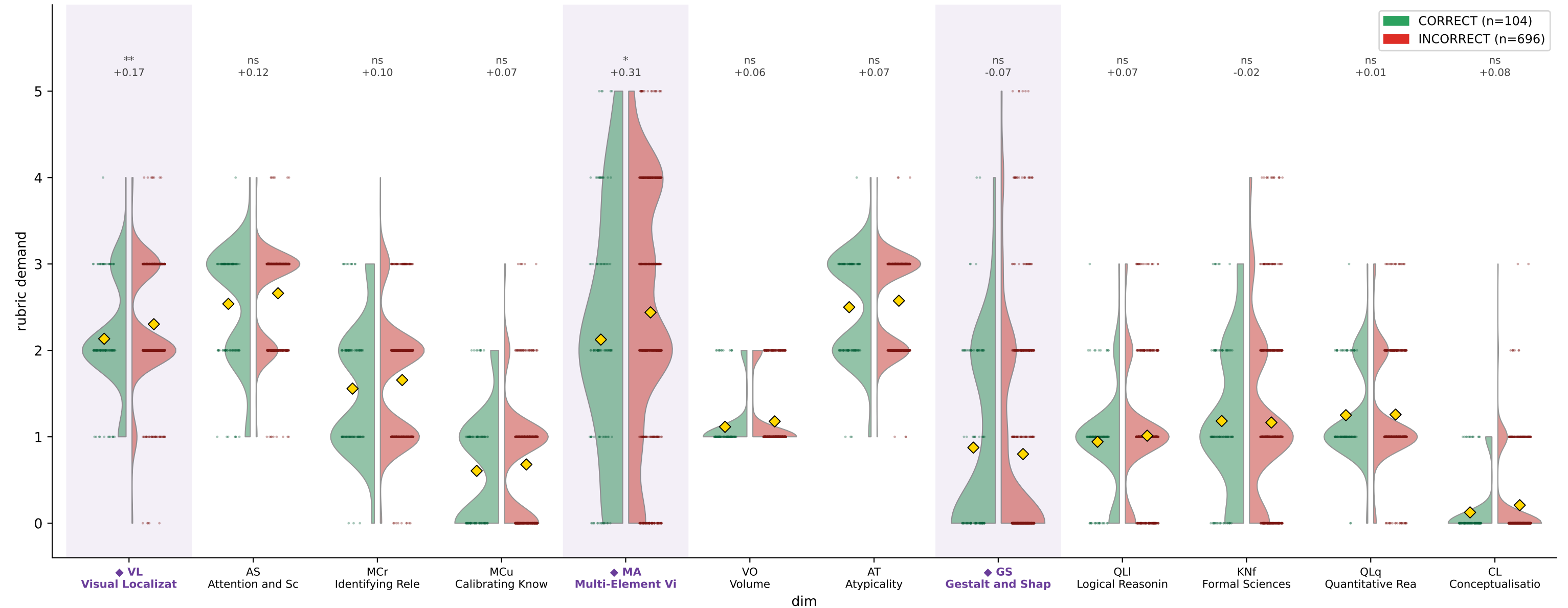
CharXiv DeLeAn demand by reasoning correctness — ChartGemma (train)
