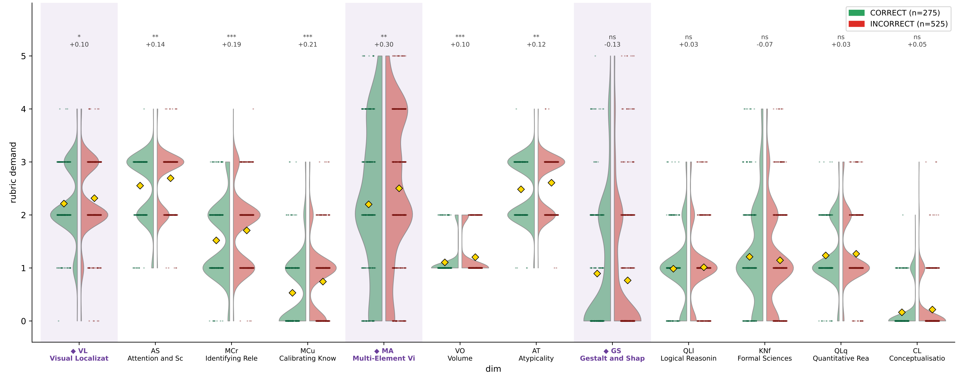
CharXiv DeLeAn demand by reasoning correctness — InternVL2-26B (train)
