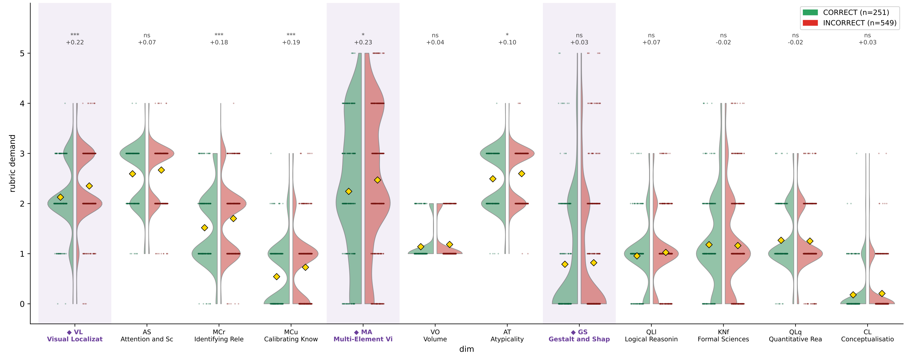
CharXiv DeLeAn demand by reasoning correctness — Phi-3-Vision (train)
