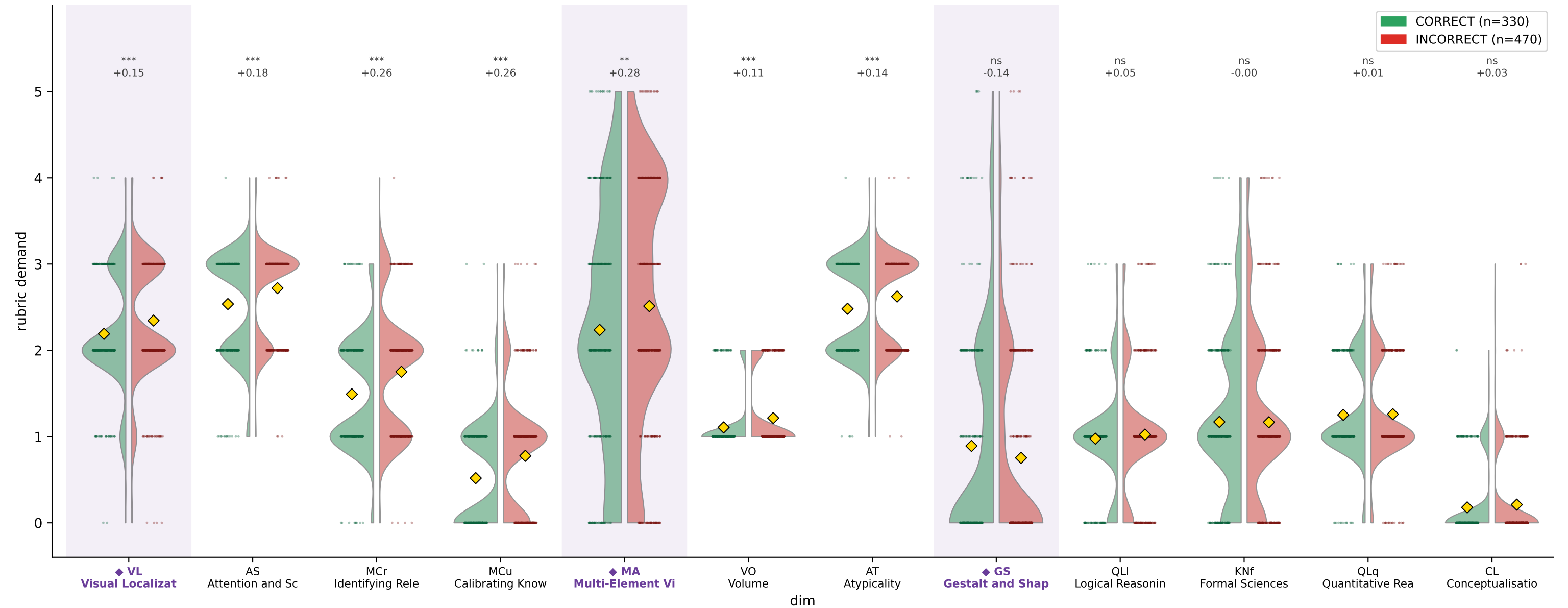
CharXiv DeLeAn demand by reasoning correctness — InternVL2-Pro (train)
