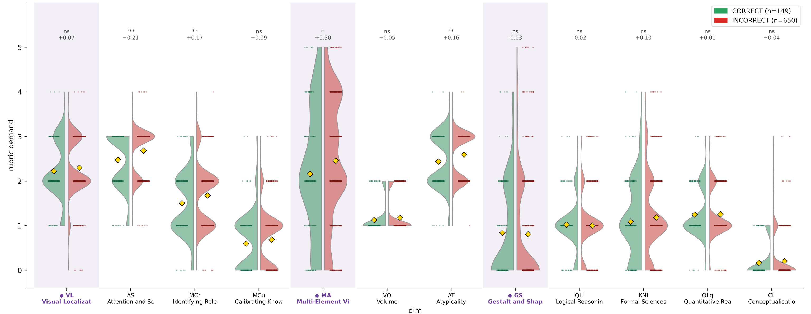
CharXiv DeLeAn demand by reasoning correctness — InternLM-XComposer2 (train)
