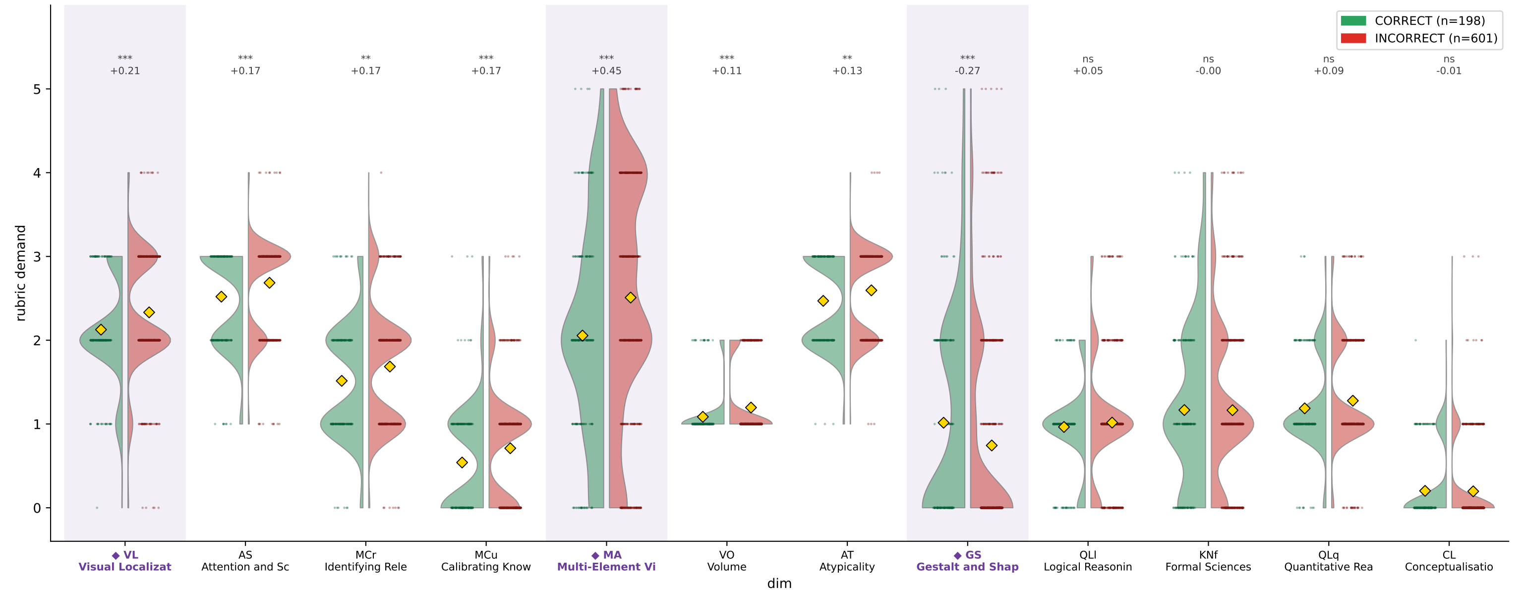
CharXiv DeLeAn demand by reasoning correctness — Mini-Gemini-HD-Yi-34B (train)
