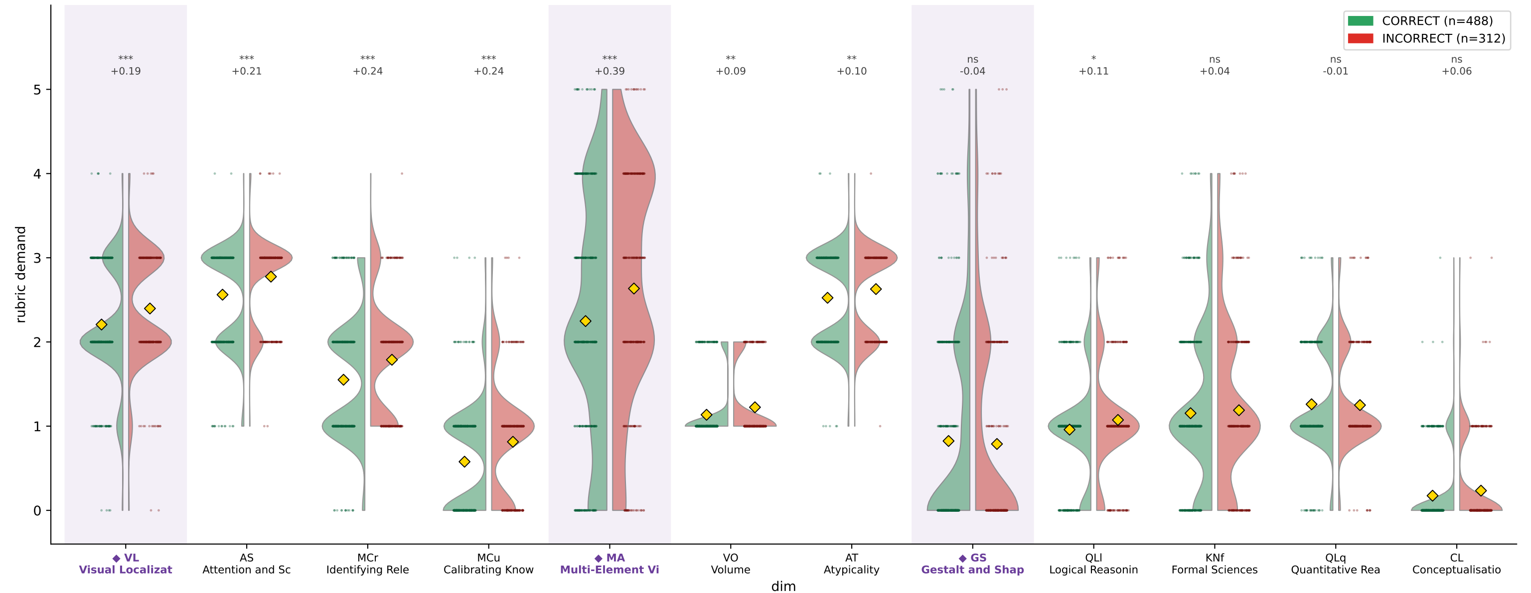
CharXiv DeLeAn demand by reasoning correctness — Claude-3-5-Sonnet (train)
