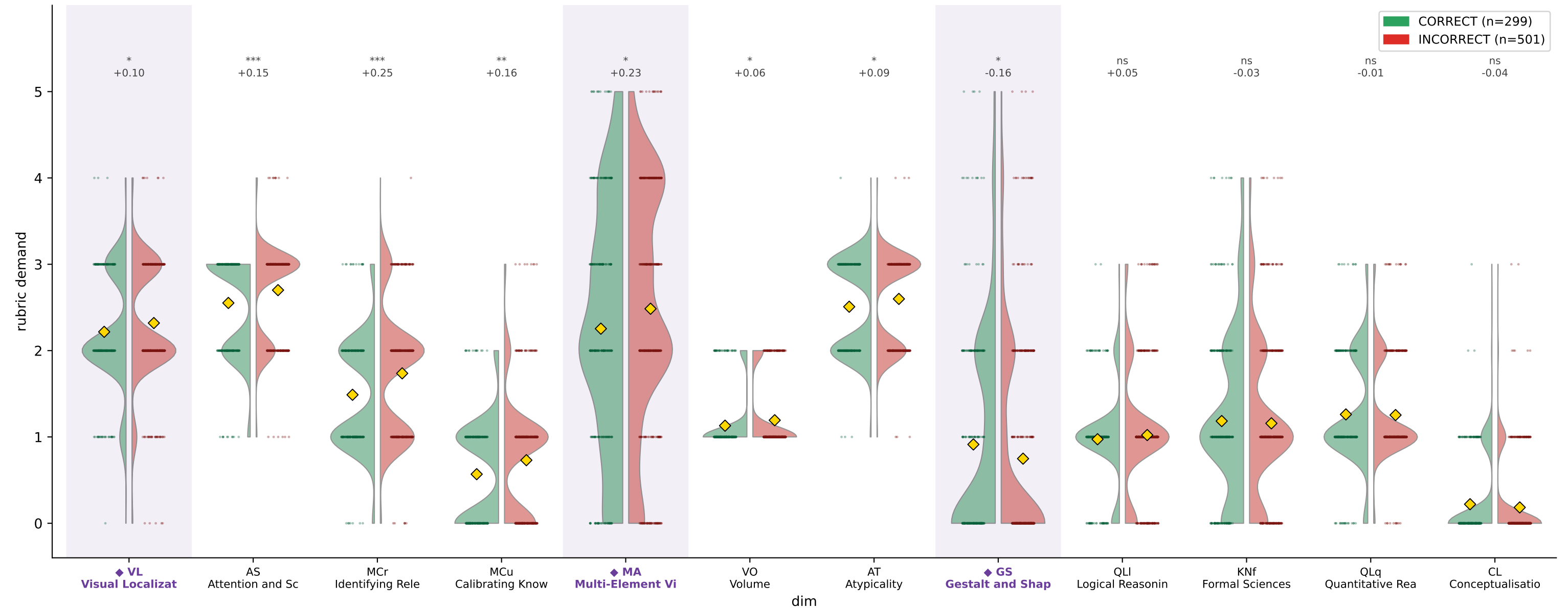
CharXiv DeLeAn demand by reasoning correctness — GPT-4V-Turbo (train)
