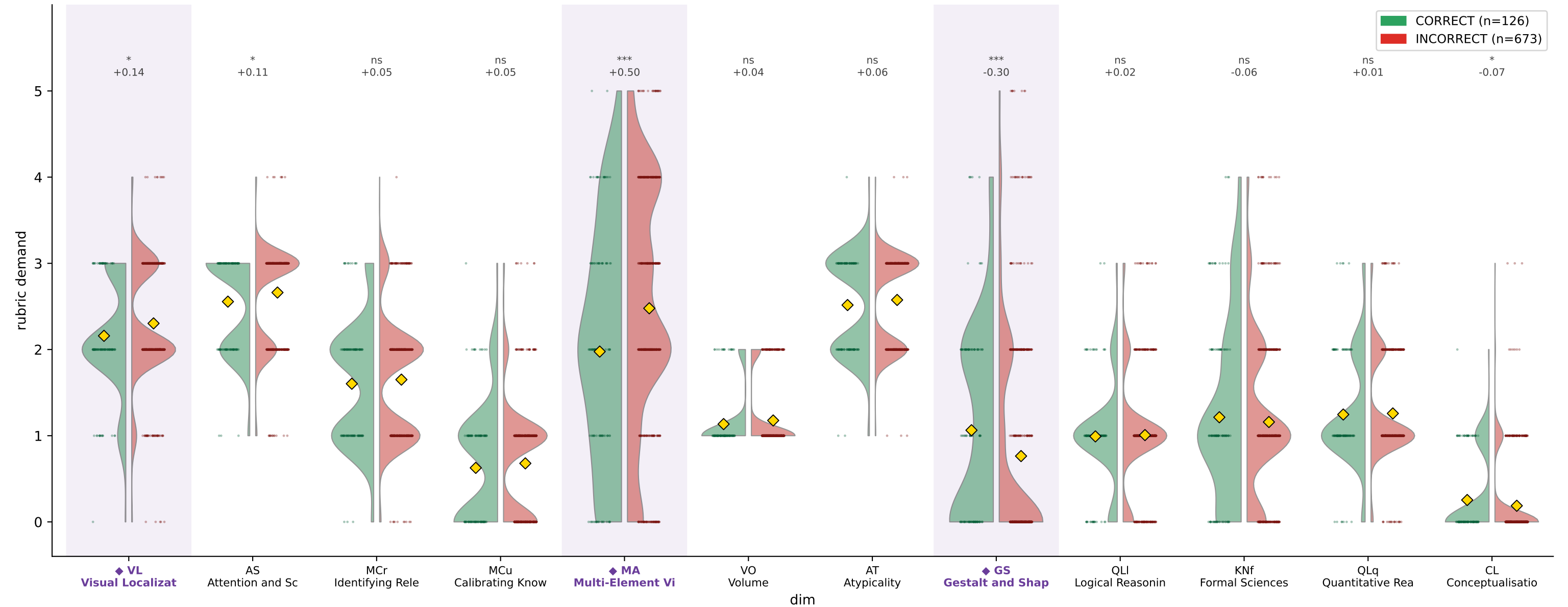
CharXiv DeLeAn demand by reasoning correctness — Qwen-VL-Plus (train)
