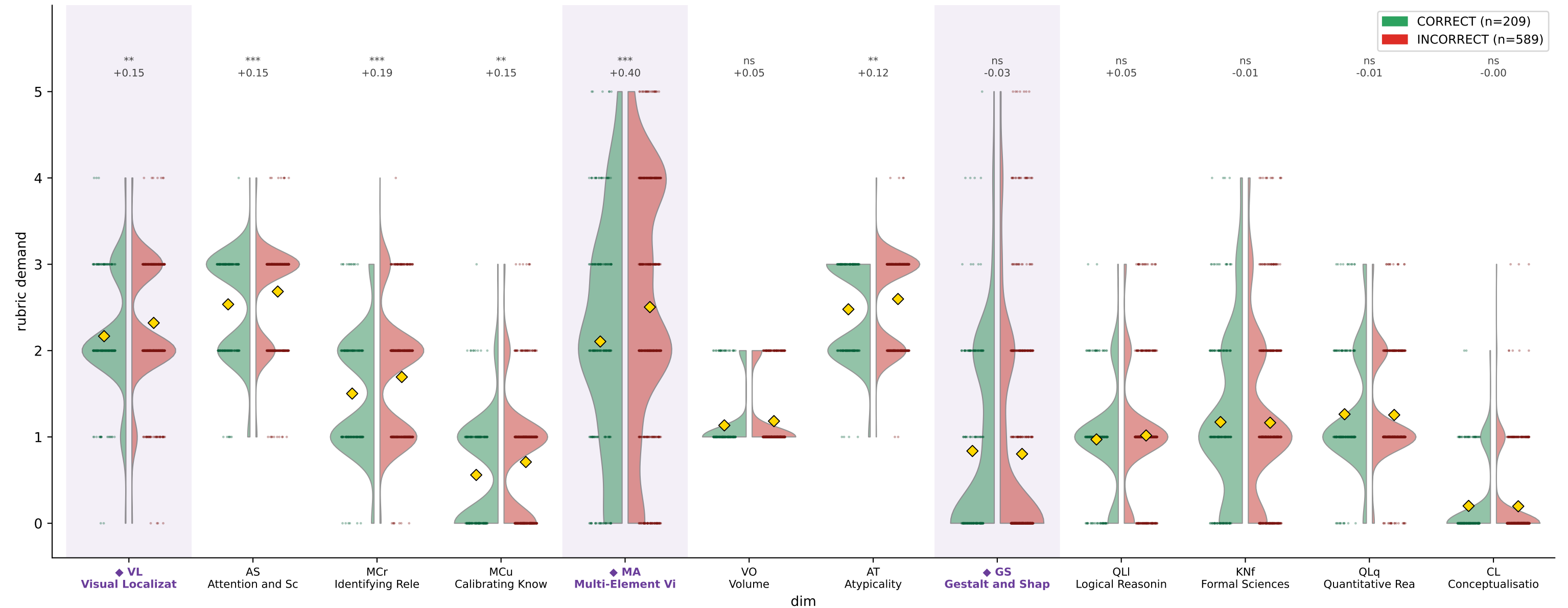
CharXiv DeLeAn demand by reasoning correctness — Reka-Flash (train)
