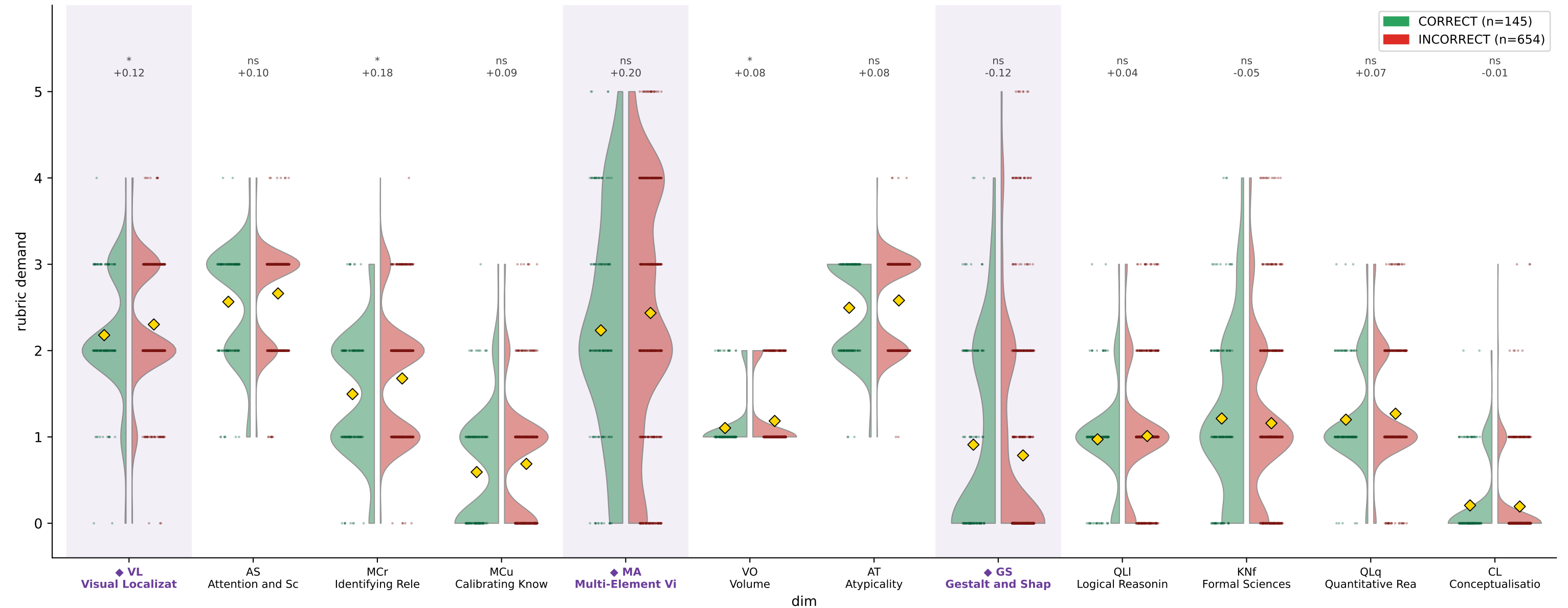
CharXiv DeLeAn demand by reasoning correctness — MiniCPM-V2 (train)
