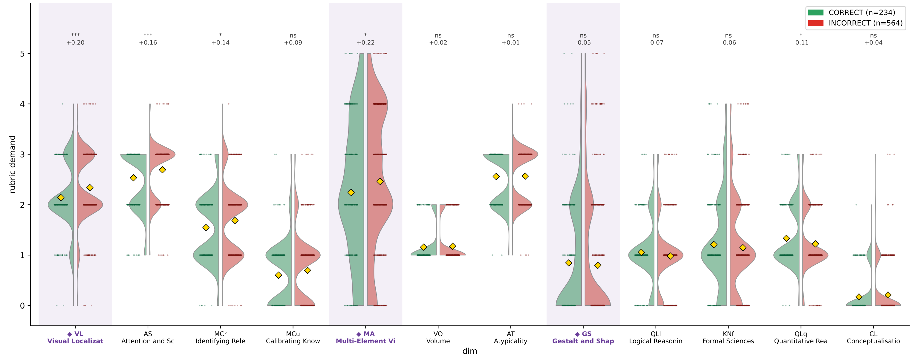
CharXiv DeLeAn demand by reasoning correctness — Reka-Core (train)
