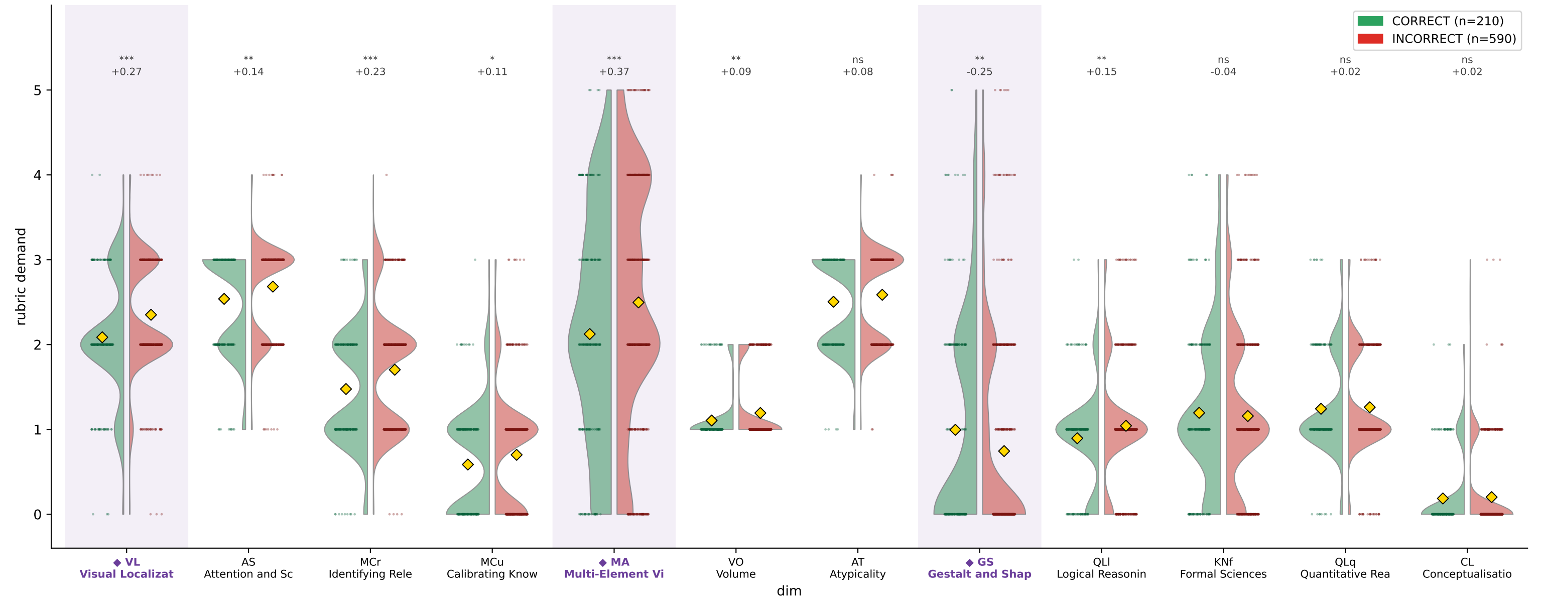
CharXiv DeLeAn demand by reasoning correctness — Cambrian-34B (train)
