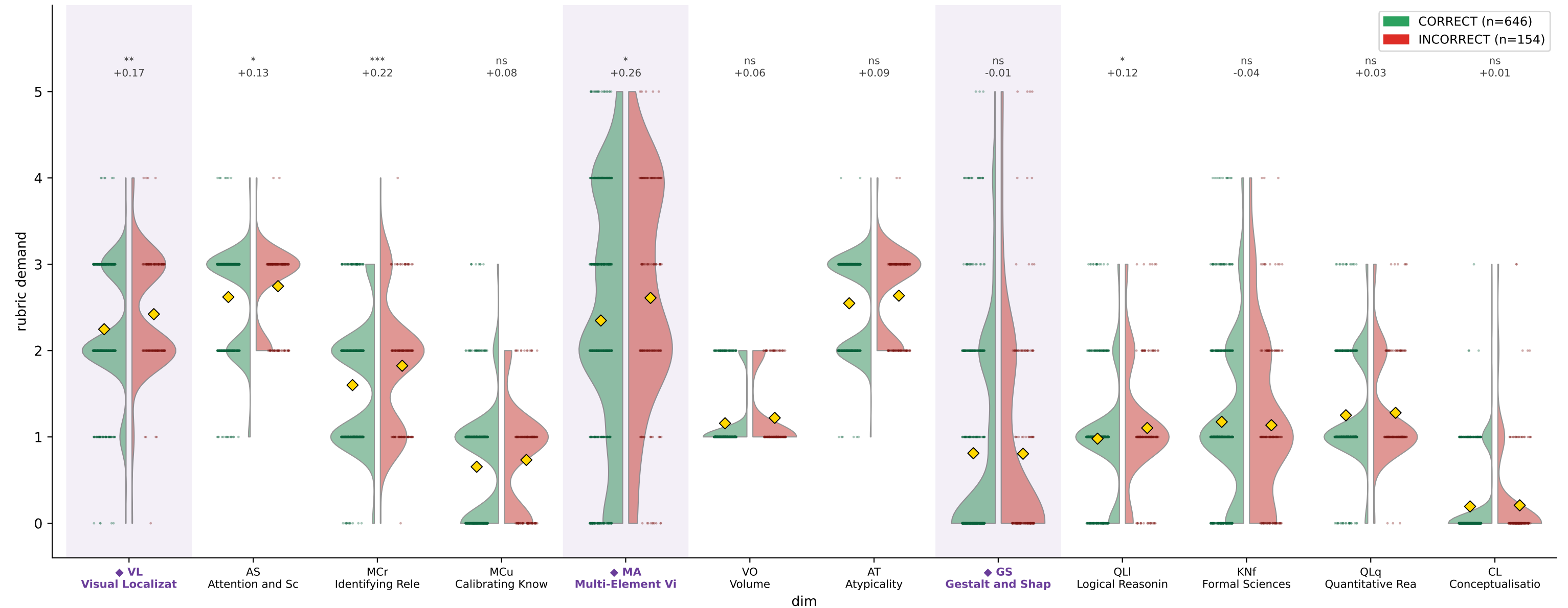
CharXiv DeLeAn demand by reasoning correctness — Human (train)
