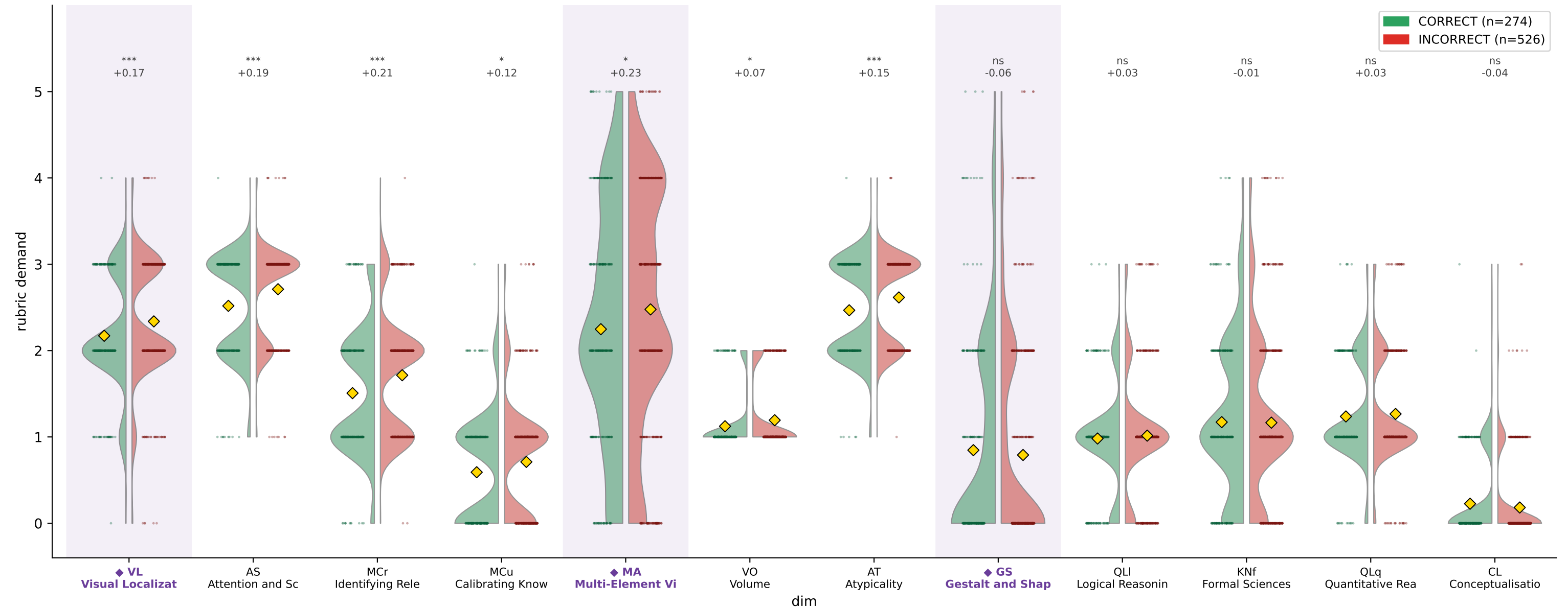
CharXiv DeLeAn demand by reasoning correctness — GPT-4o-mini (train)
