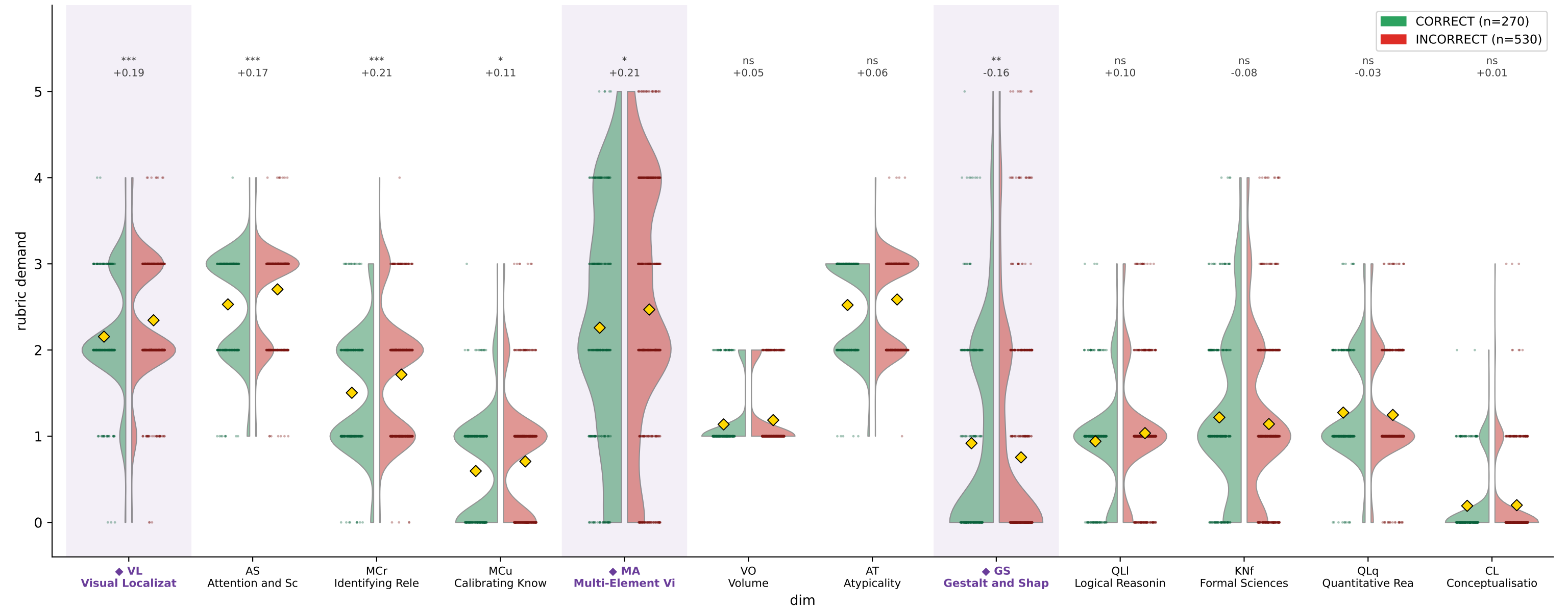
CharXiv DeLeAn demand by reasoning correctness — Claude-3-Sonnet (train)
