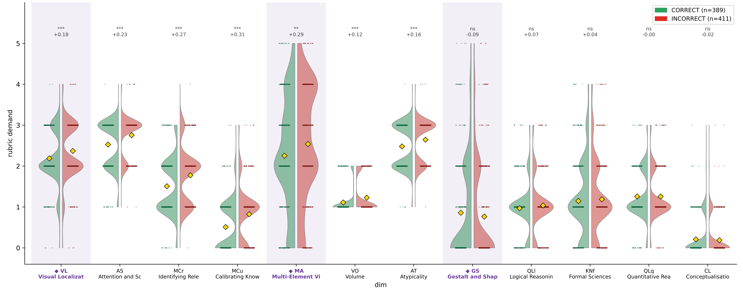
CharXiv DeLeAn demand by reasoning correctness — GPT-4o (train)
