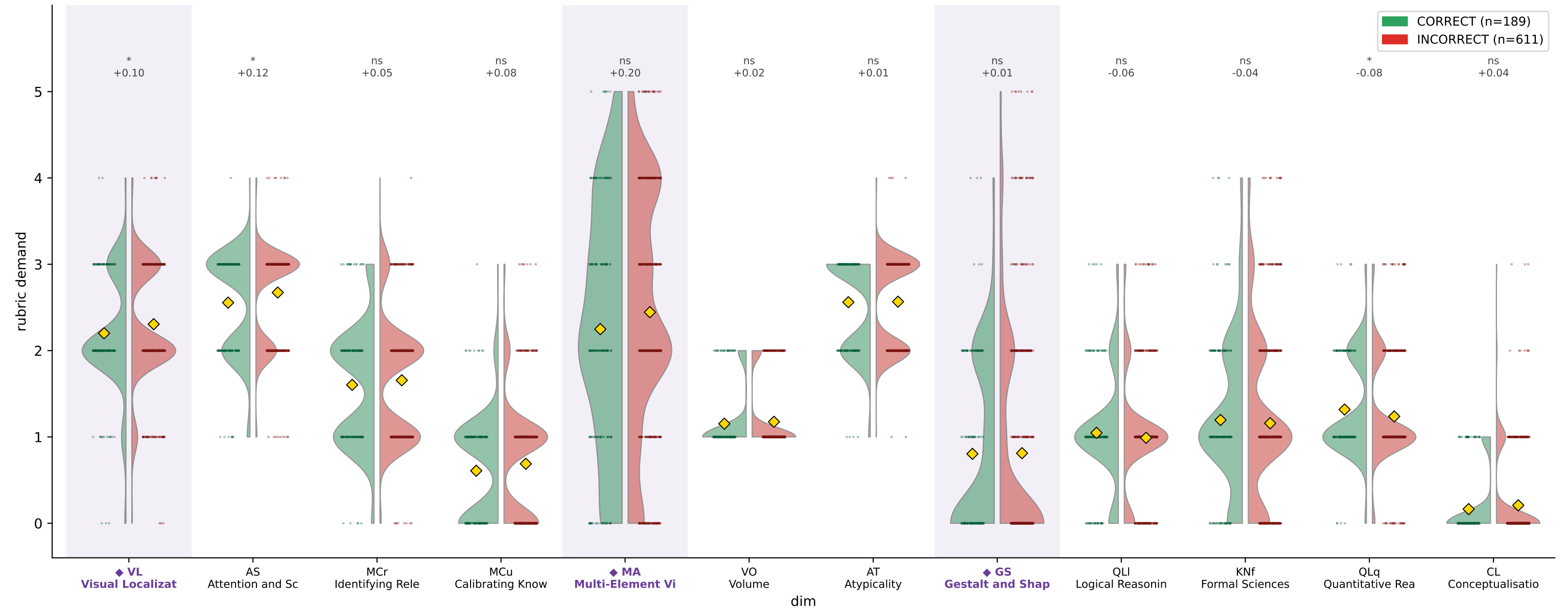
CharXiv DeLeAn demand by reasoning correctness — Reka-Edge (train)
