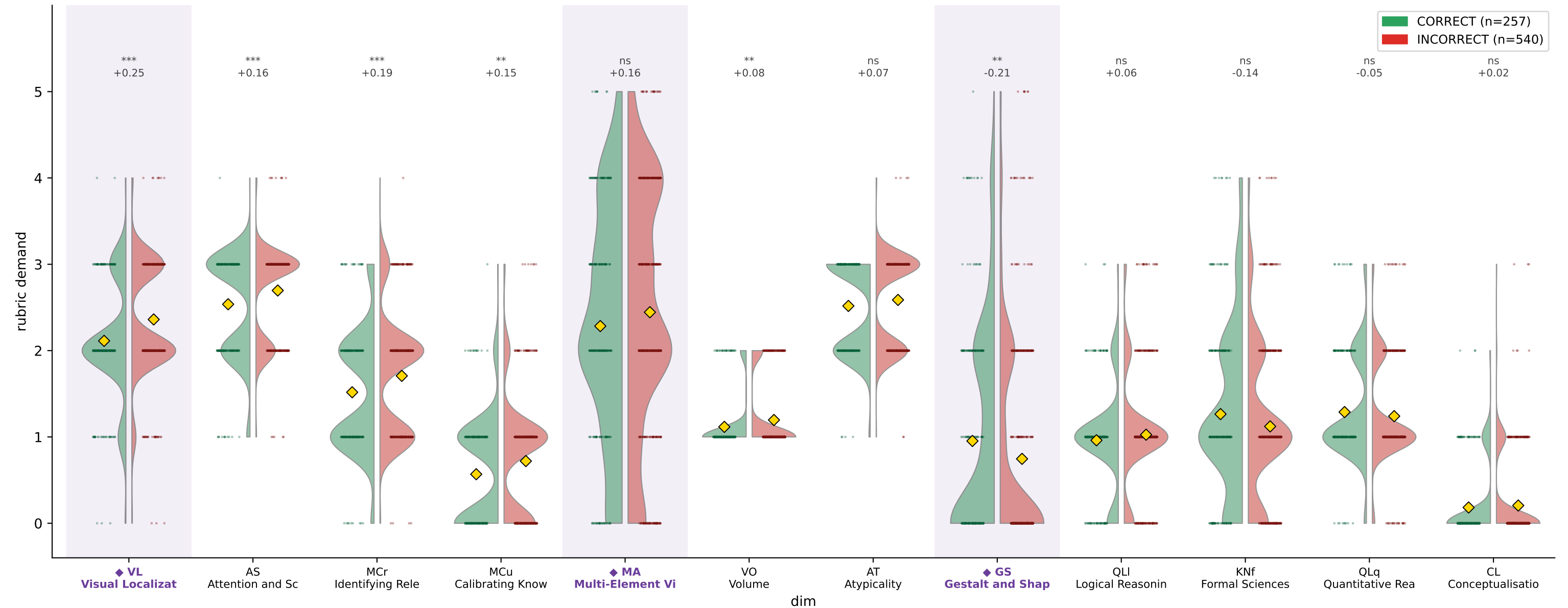
CharXiv DeLeAn demand by reasoning correctness — Claude-3-Haiku (train)
