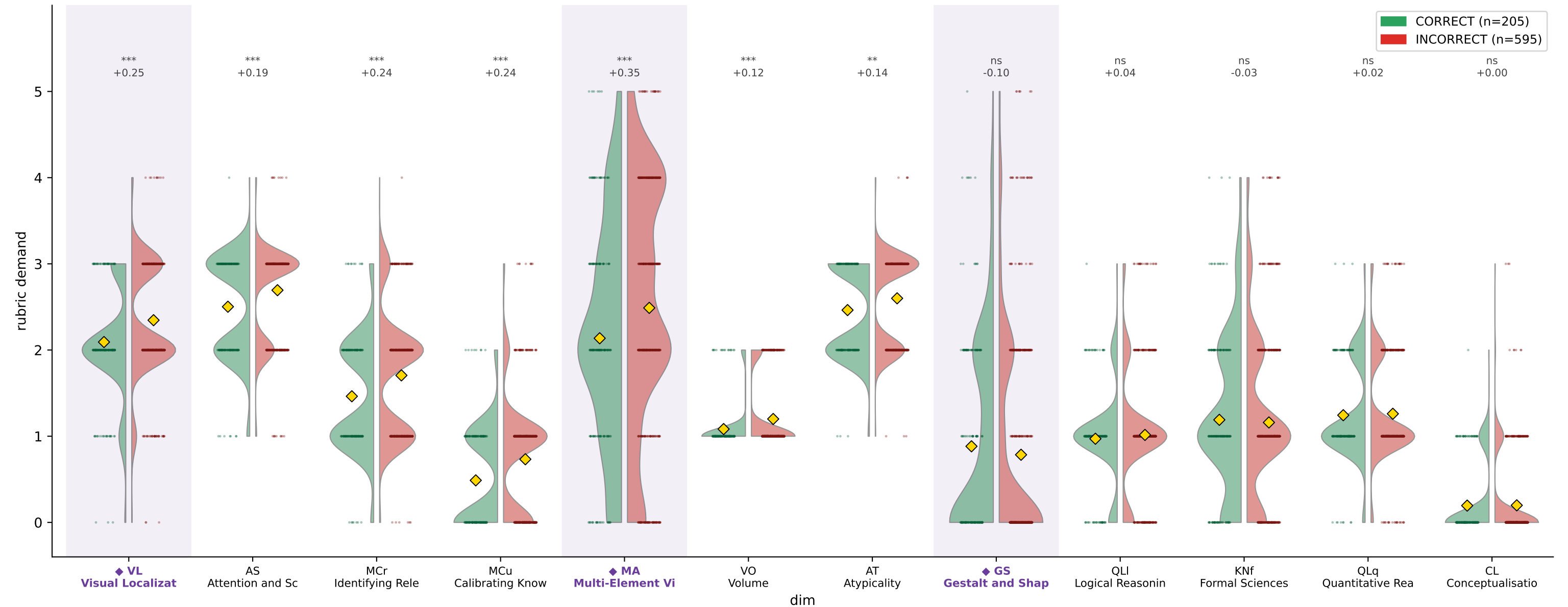
CharXiv DeLeAn demand by reasoning correctness — Qwen-VL-Max (train)
