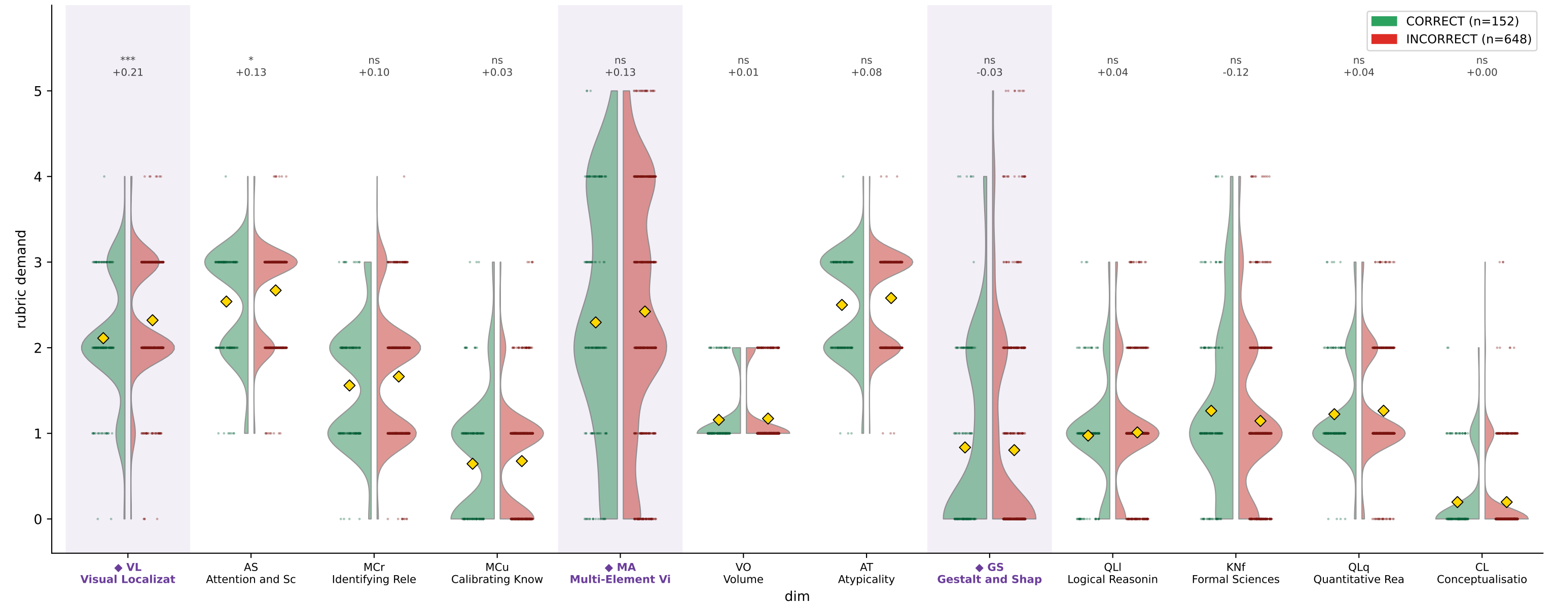
CharXiv DeLeAn demand by reasoning correctness — IDEFICS-2 (train)
