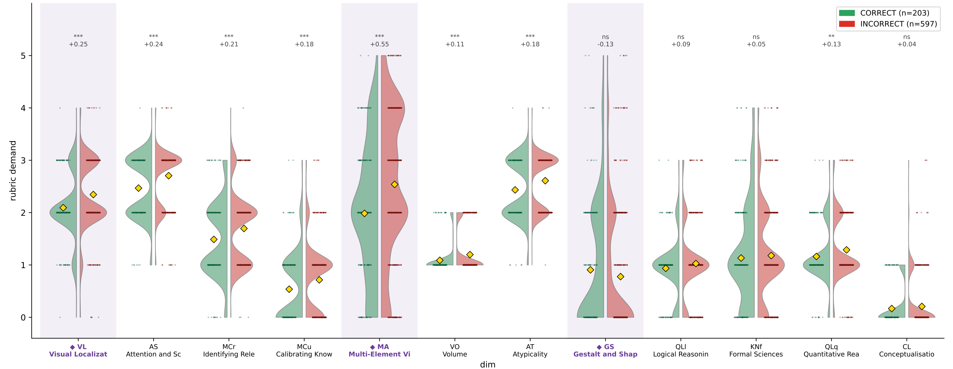
CharXiv DeLeAn demand by reasoning correctness — MiniCPM-V2-5 (train)
