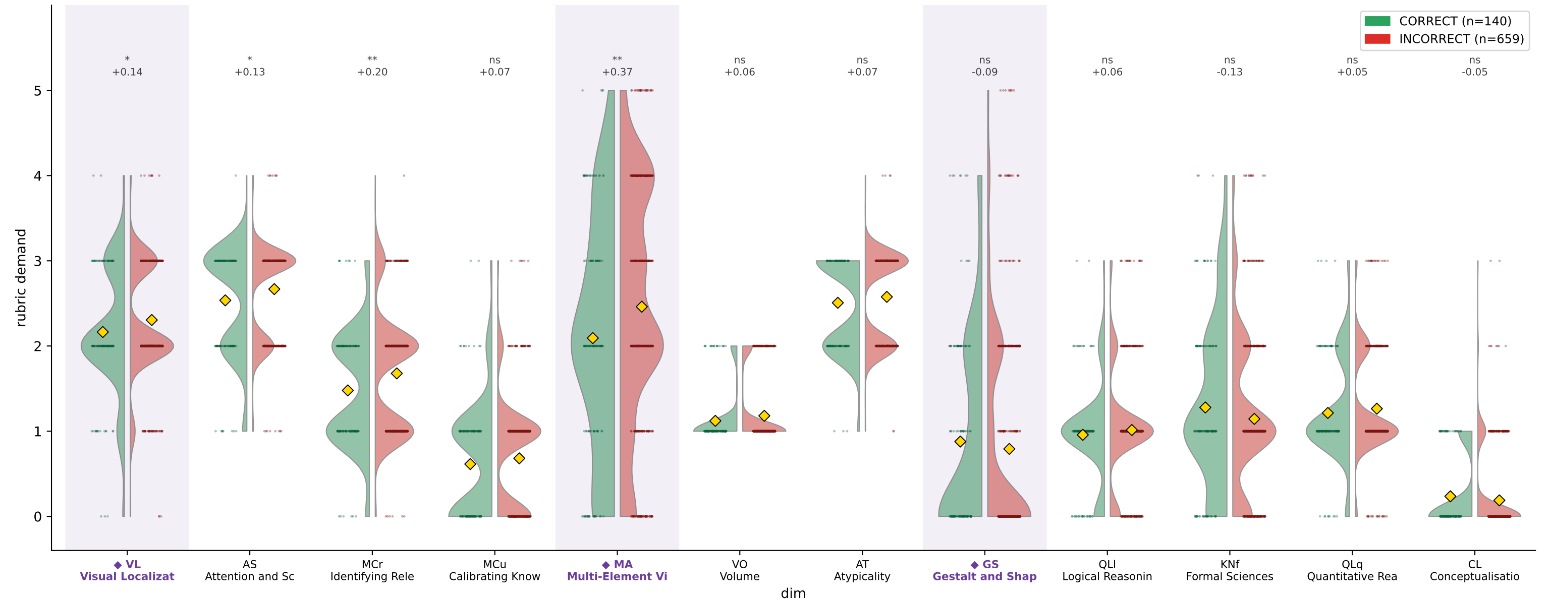
CharXiv DeLeAn demand by reasoning correctness — DeepSeek-VL (train)
