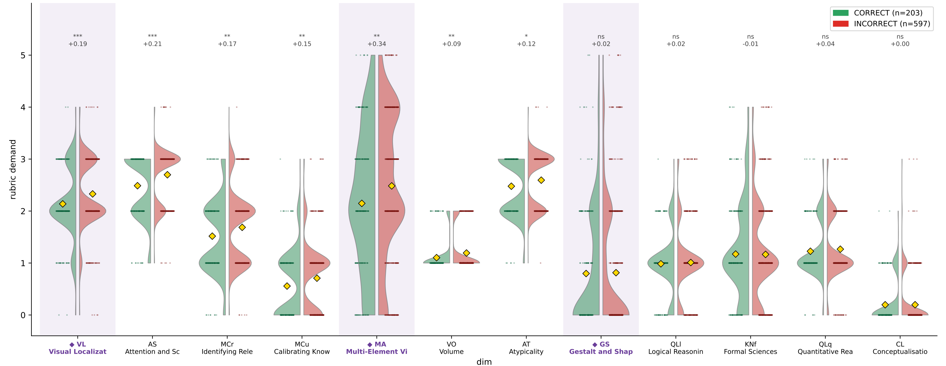
CharXiv DeLeAn demand by reasoning correctness — InternLM-XComposer2-4KHD (train)
