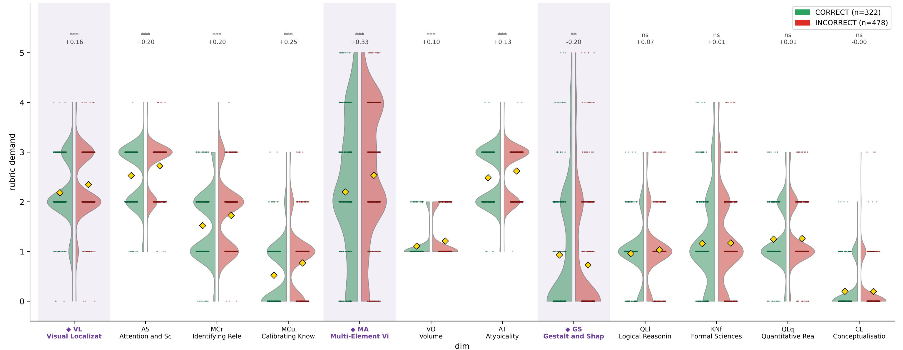
CharXiv DeLeAn demand by reasoning correctness — InternVL2-76B (train)
