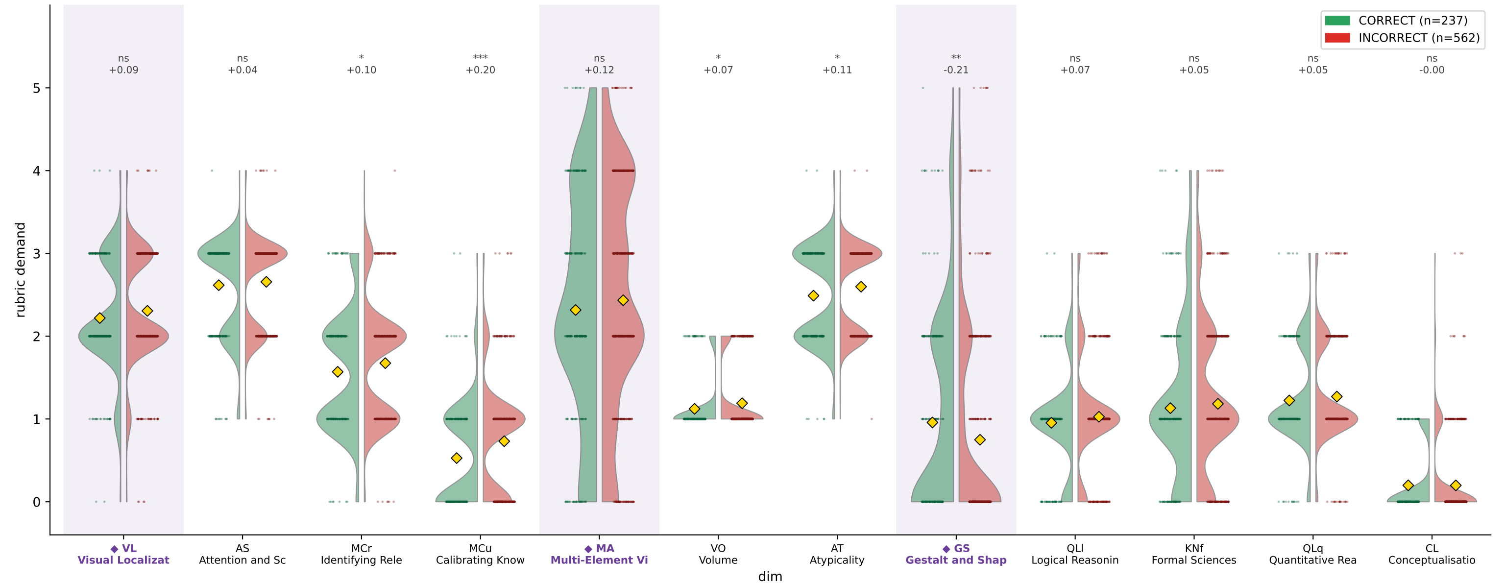
CharXiv DeLeAn demand by reasoning correctness — InternVL-Chat-V1-5 (train)
