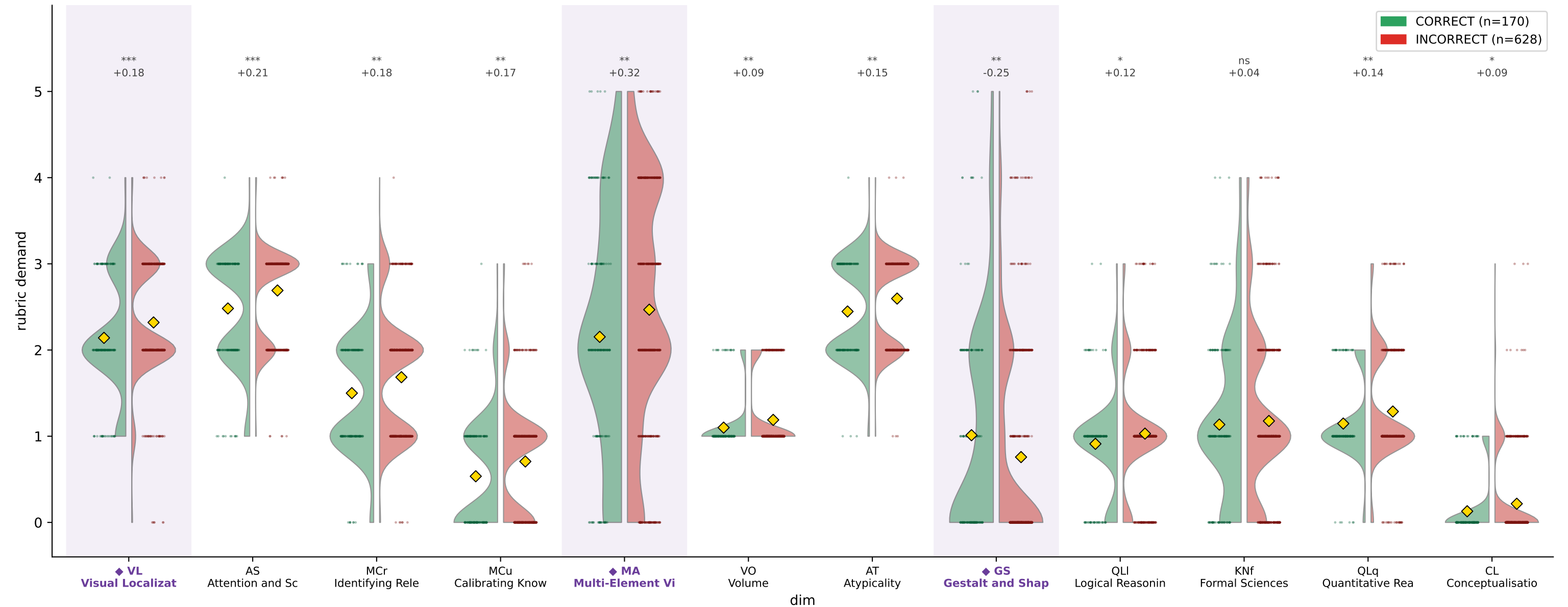
CharXiv DeLeAn demand by reasoning correctness — LLaVA-1-6-Yi-34B (train)
