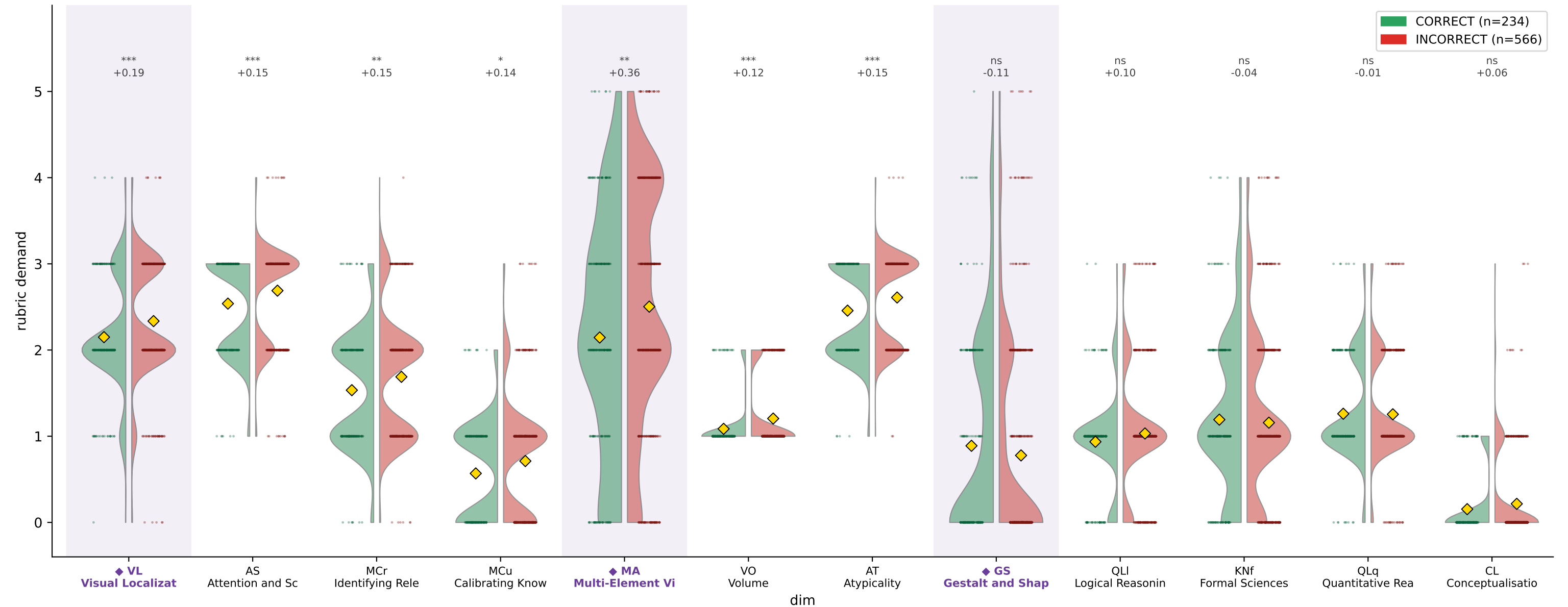
CharXiv DeLeAn demand by reasoning correctness — Ovis1.5-Llama3-8B (train)
