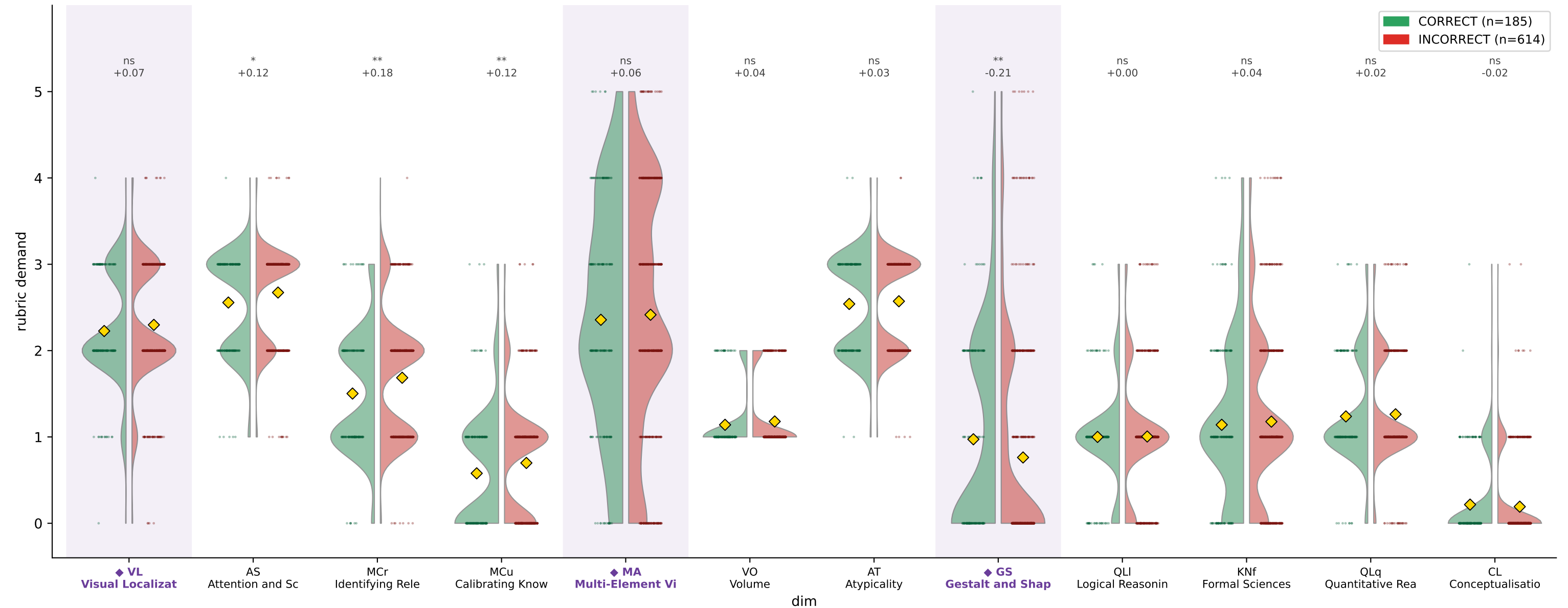
CharXiv DeLeAn demand by reasoning correctness — Gemini-1.0-Pro-Vision (train)
