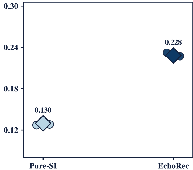
SRec-to-LLM RBO@20
