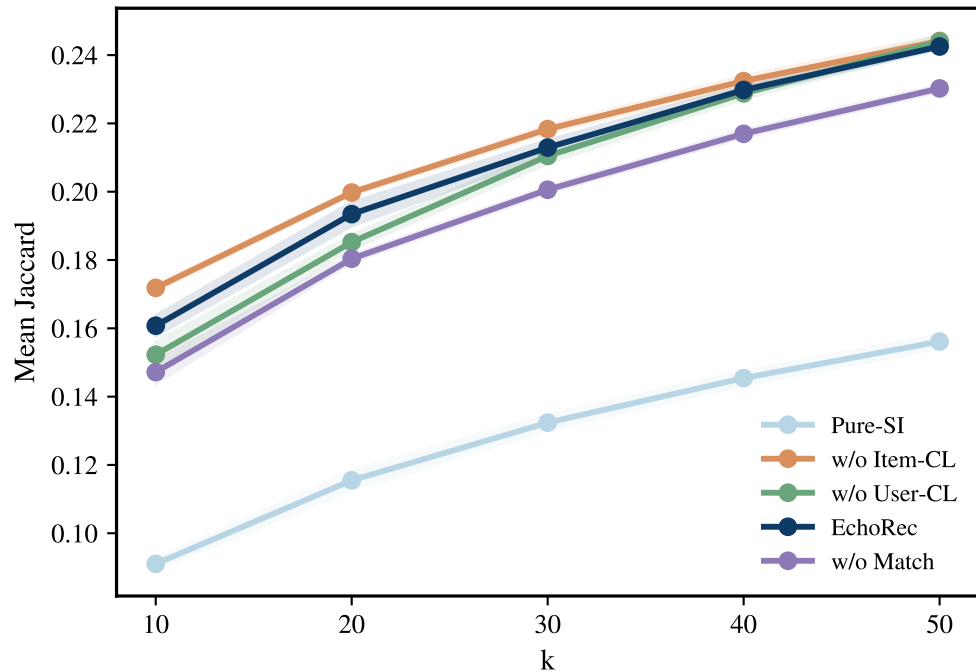
Structure Transfer Jaccard@k
