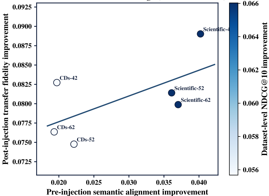
Cross-dataset mechanism bridge (Pearson = 0.634)
