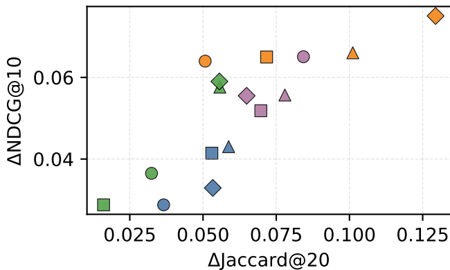
Spearman \rho=0.788
