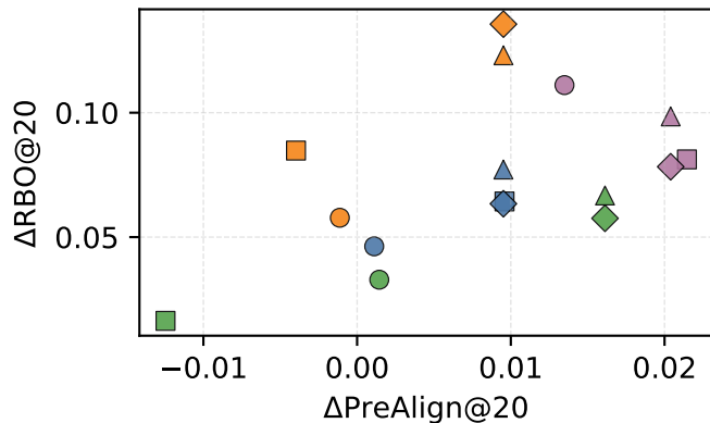
Spearman \rho=0.444
