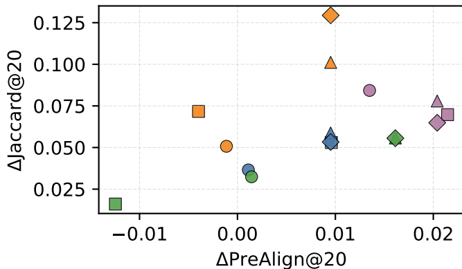
Spearman \rho=0.487
