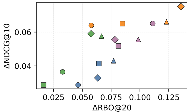
Spearman \rho=0.756
