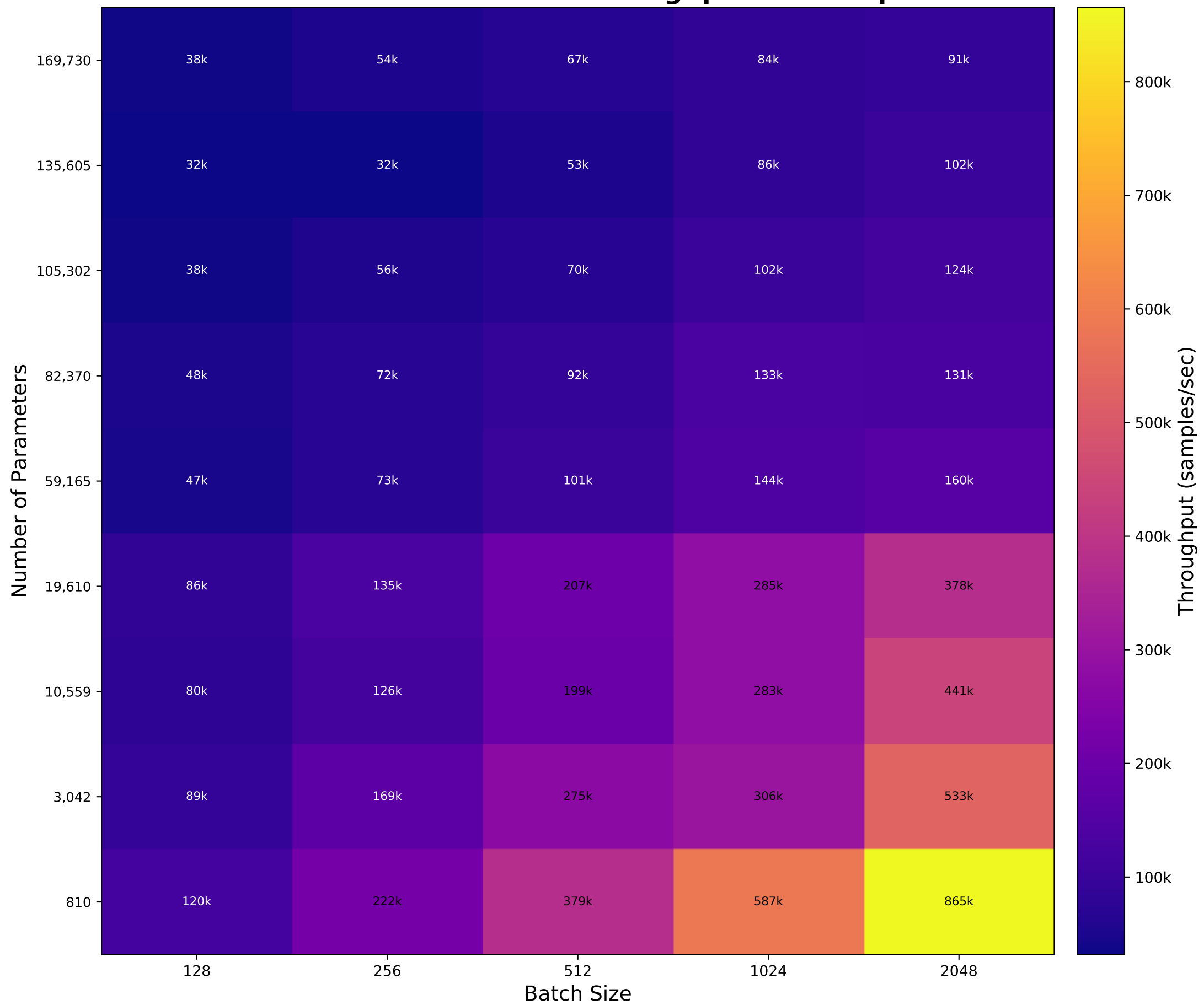
TetrahedronPairNet: Throughput Heatmap
