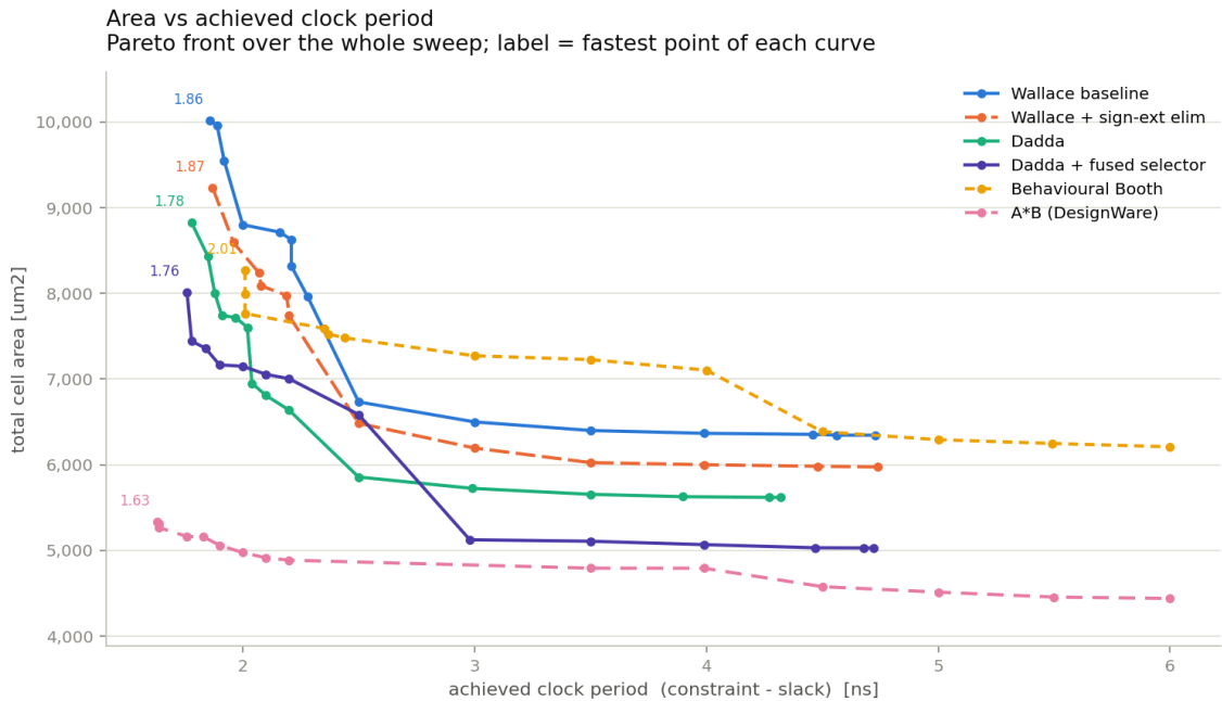
Figure 2: Area against derived zero-slack period. Each curve is the Pareto front of one variant over the whole 21-point sweep; dominated runs are omitted. Lower and further left is better.
