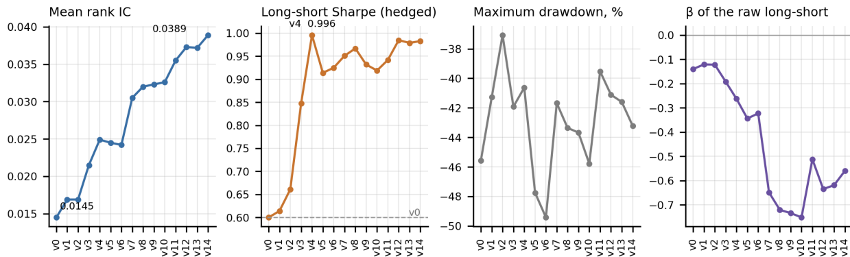
Figure 4. The ratchet by version. Mean IC rises at almost every acceptance, as the residual bar makes likely. The hedged long-short Sharpe peaks at v4 and stays below that peak through the later ladders. The full-window \beta of the raw long-short falls from -0.14 to -0.75 by v10 and recovers to -0.56 as the two positive- \beta legs join; the hedge removes that exposure ex ante.
