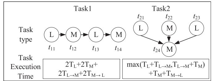
Fig. 2. The diagram of the MTO.
