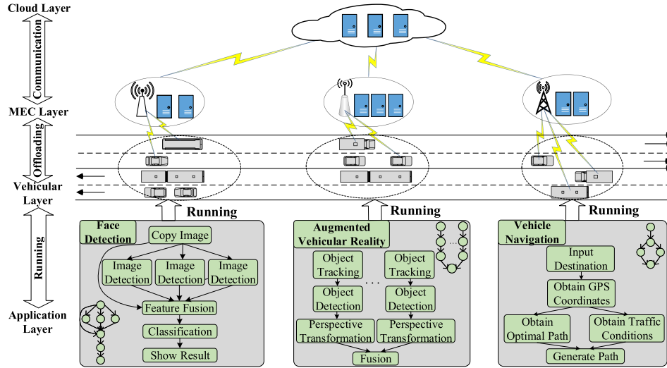
Fig. 1. The system architecture of multi-task offloading in MEC-based vehicular network.
