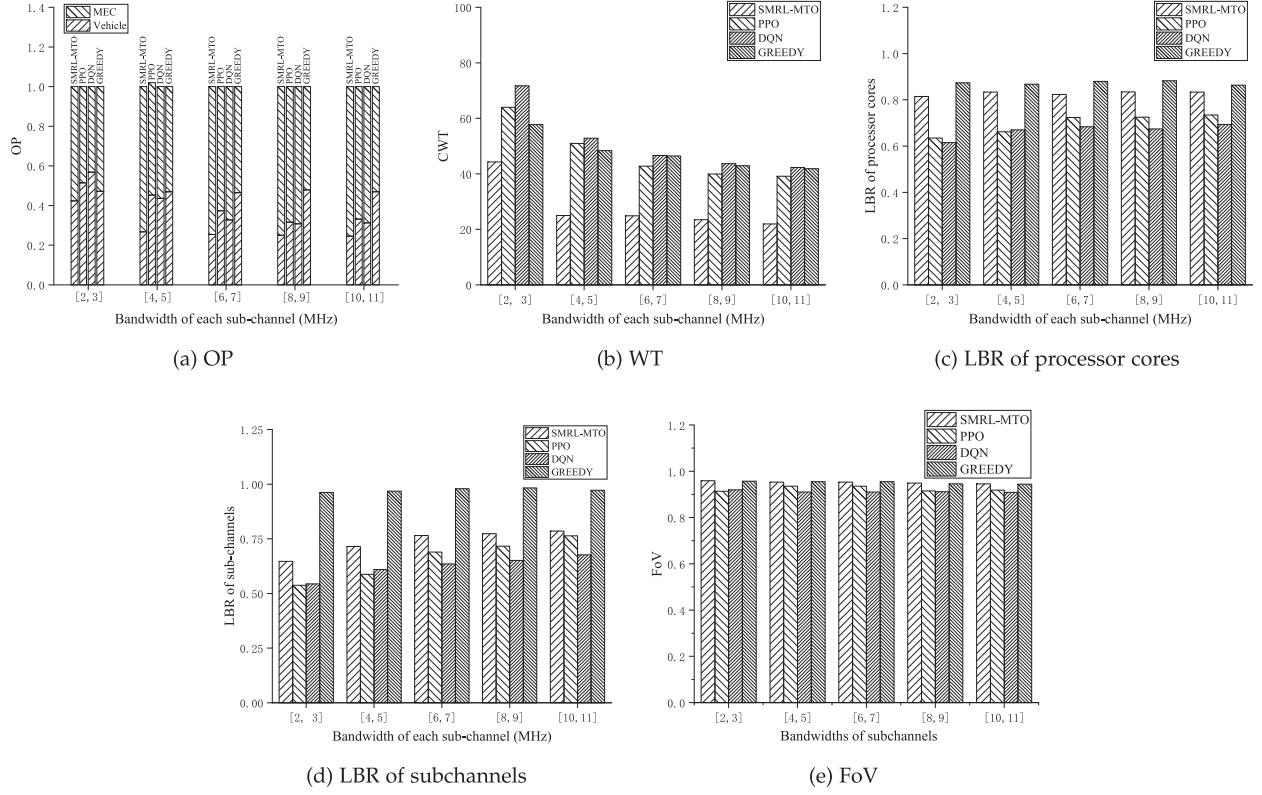
Fig. 6. The performance of four algorithms under different bandwidths of subchannels.
