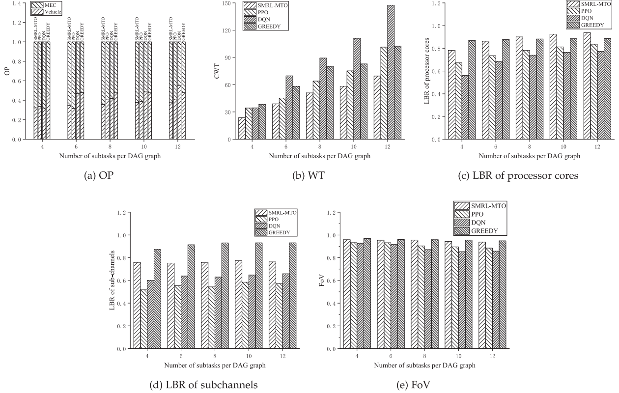
Fig. 4. The performance of four algorithms under different subtask numbers.
