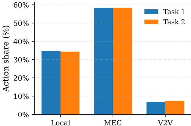
MARGO action distribution at iteration 100
